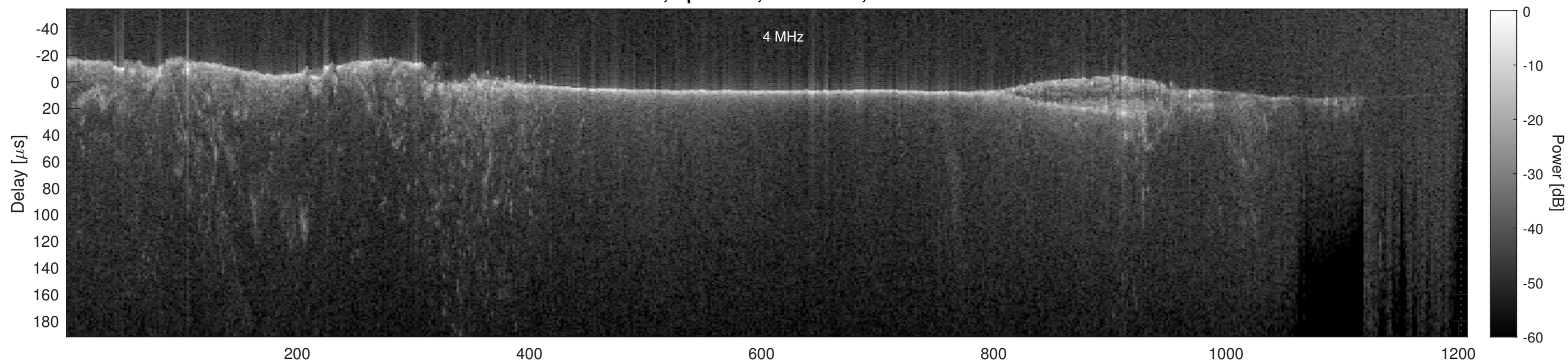
Orbit 9929, Cluttergram
