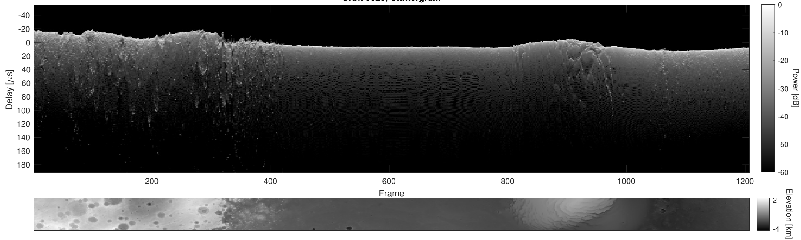
Orbit 9929, Cluttergram
