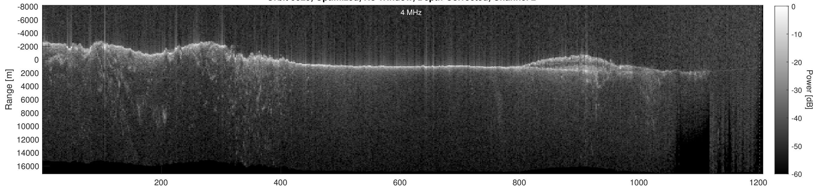
Orbit 9929, Depth-Corrected Cluttergram
