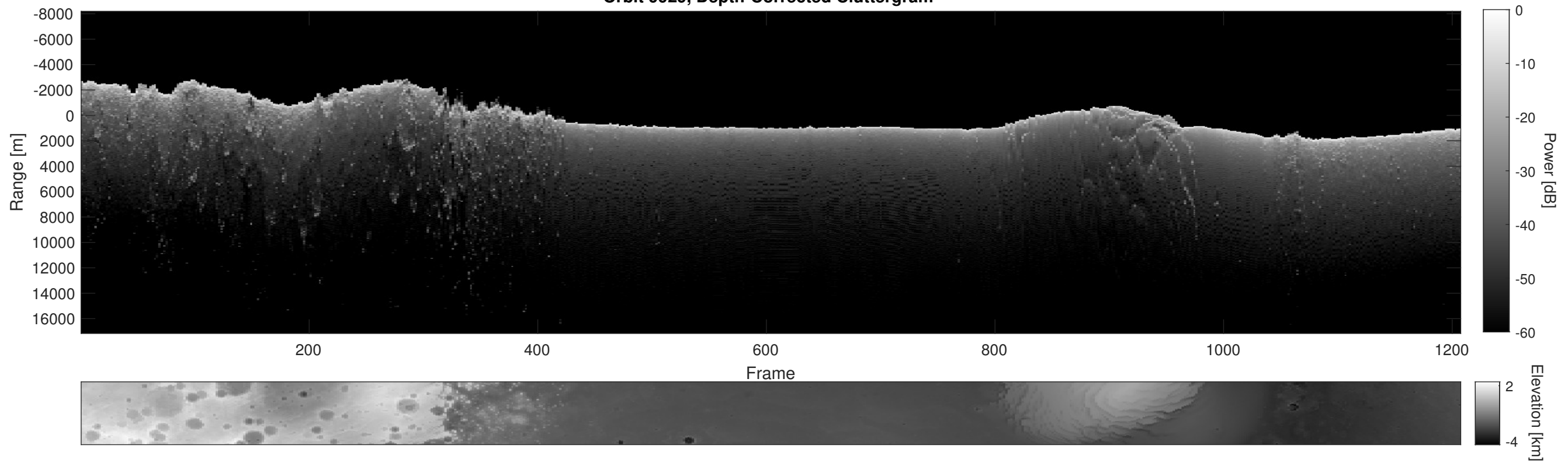
Orbit 9929, Depth-Corrected Cluttergram
