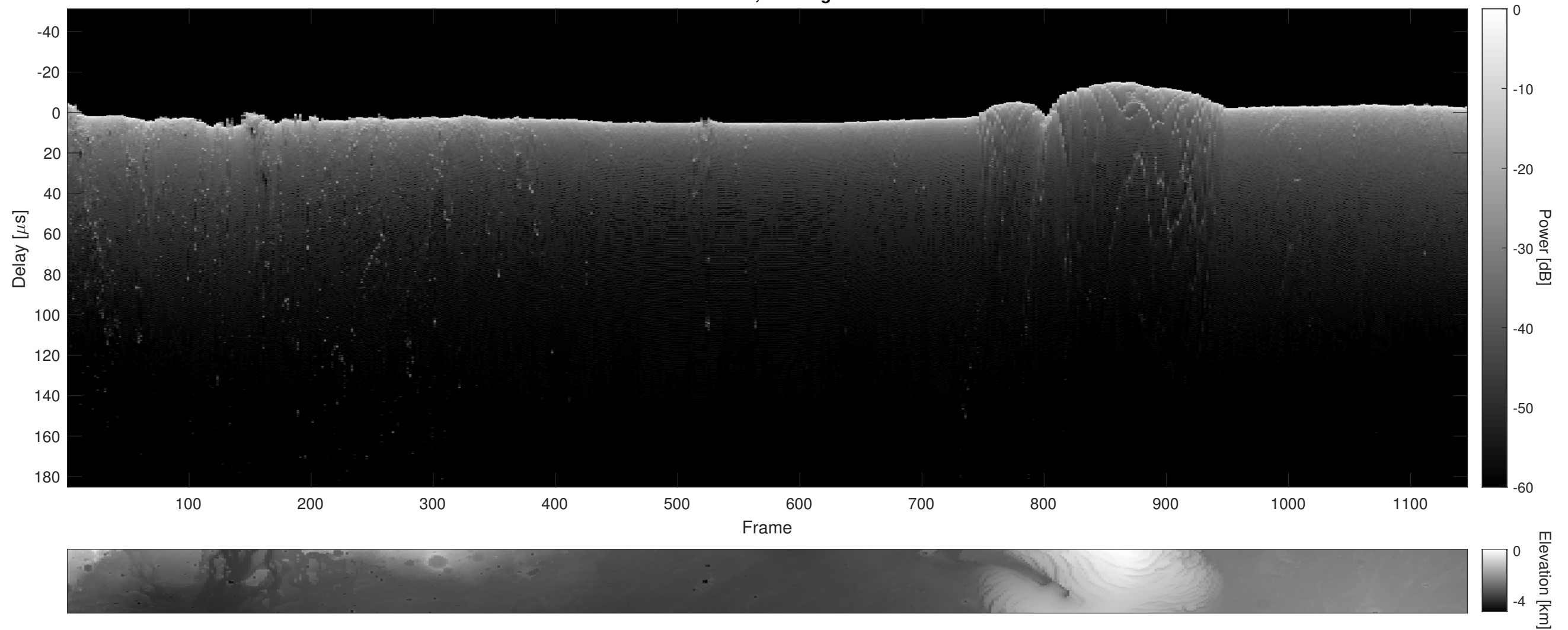
Orbit 9930, Cluttergram
