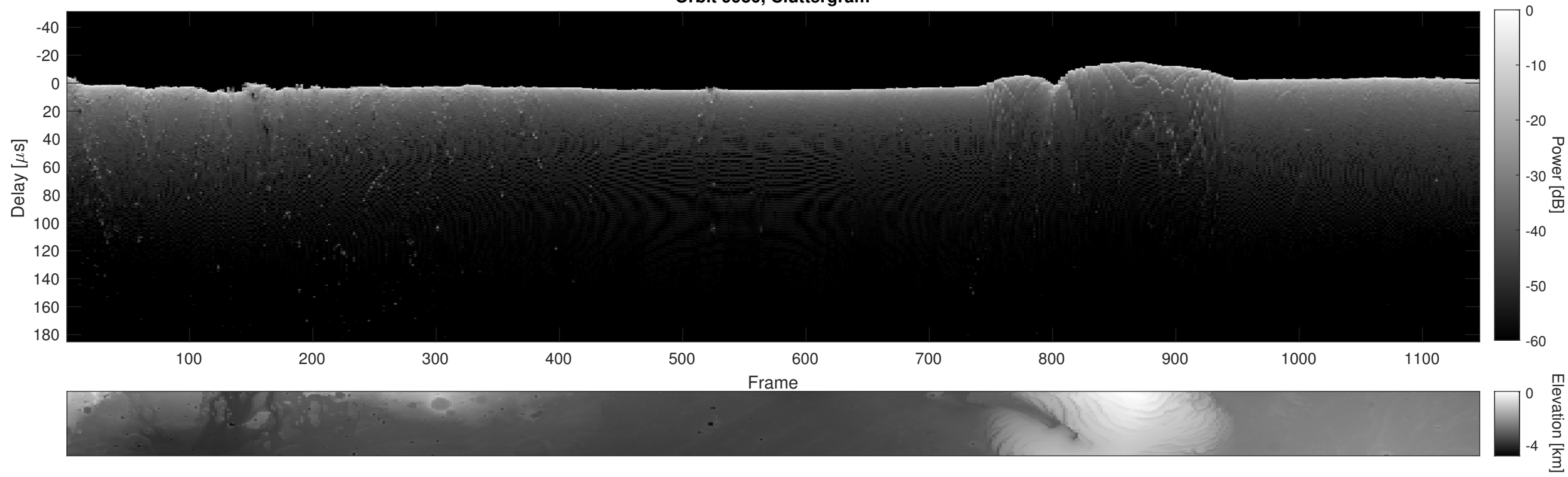
Orbit 9930, Cluttergram
