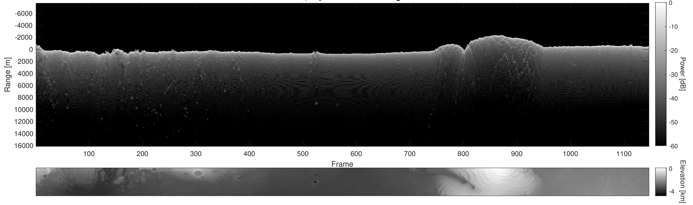
Orbit 9930, Depth-Corrected Cluttergram
