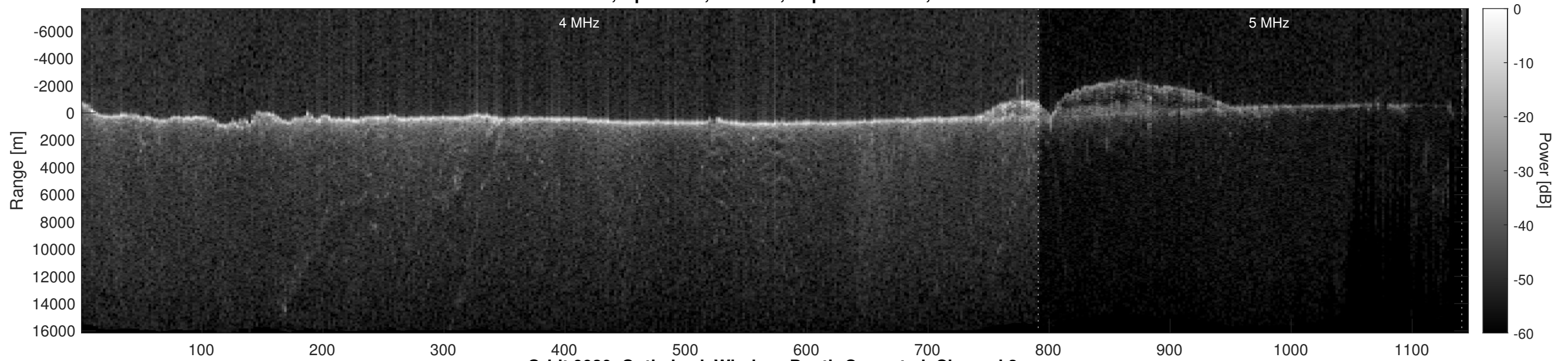
Orbit 9930, Optimized, Window, Depth-Corrected, Channel 2
