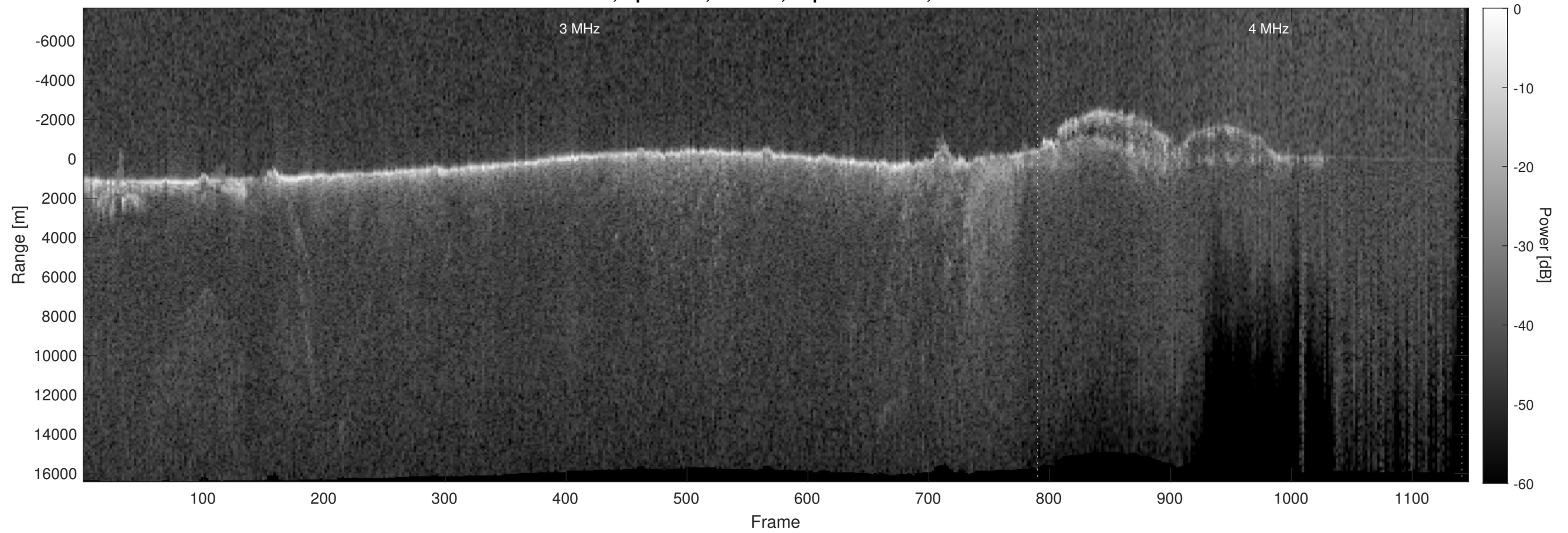
Orbit 9931, Optimized, Window, Depth-Corrected, Channel 2
