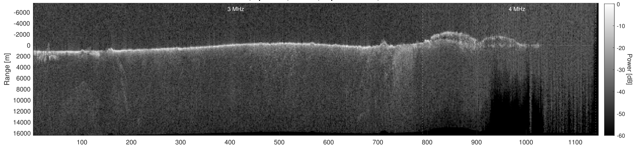
Orbit 9931, Depth-Corrected Cluttergram
