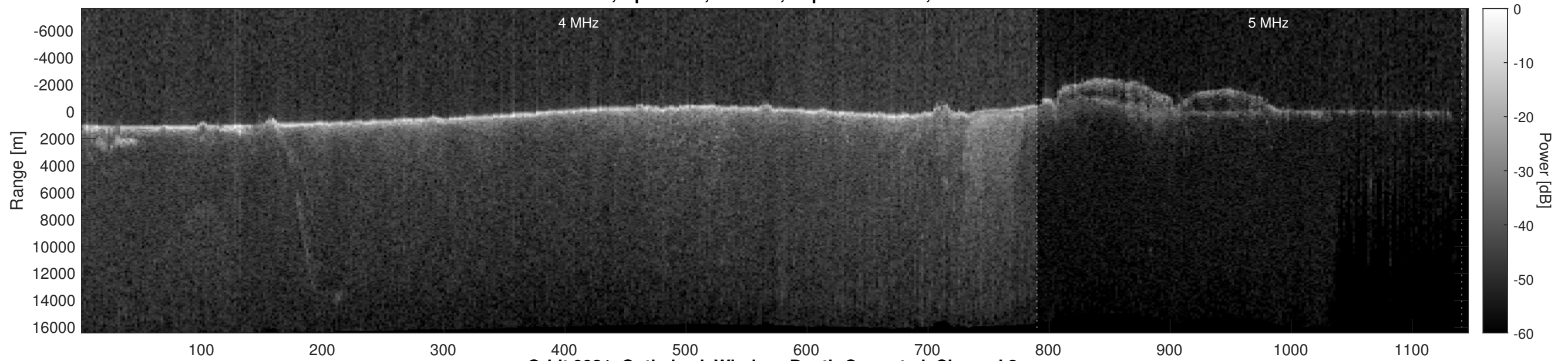
Orbit 9931, Optimized, Window, Depth-Corrected, Channel 2
