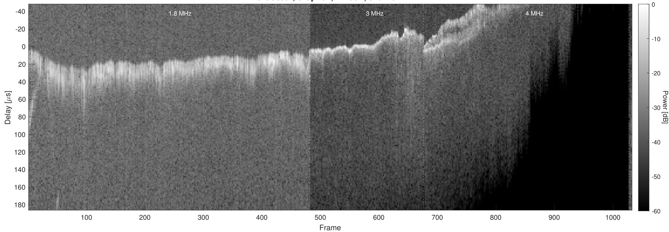
Orbit 9932, Chapman, Window, Channel 2
