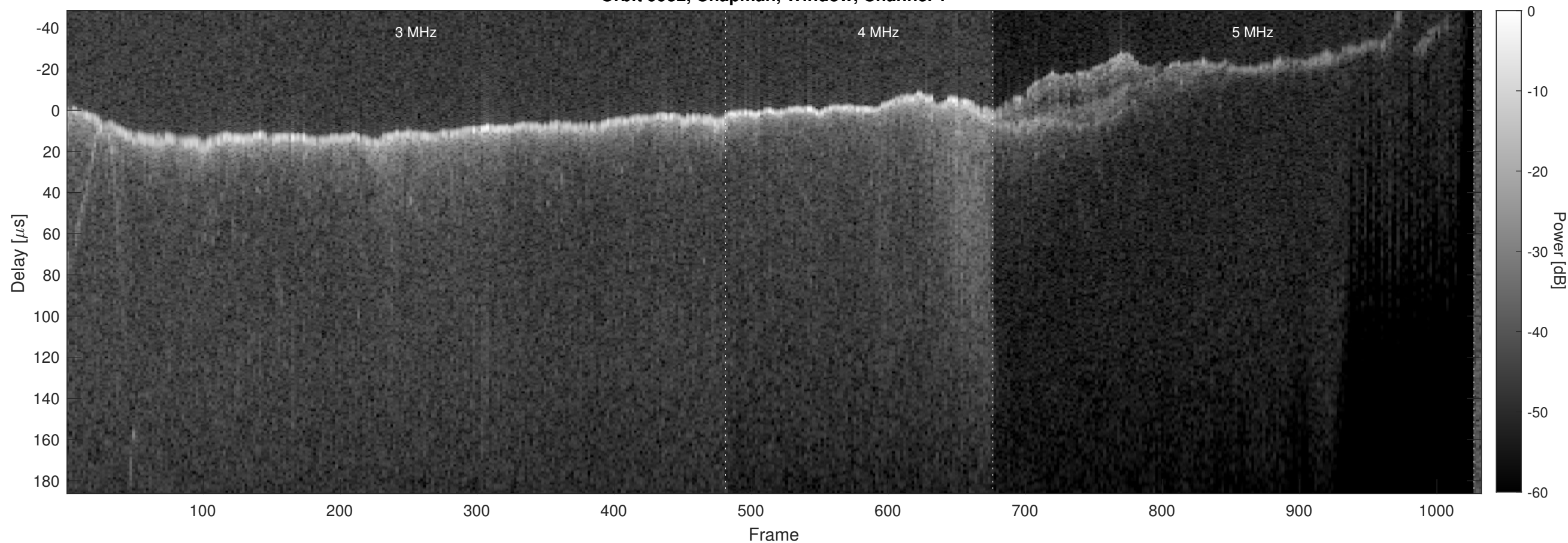
Orbit 9932, Chapman, Window, Channel 2
