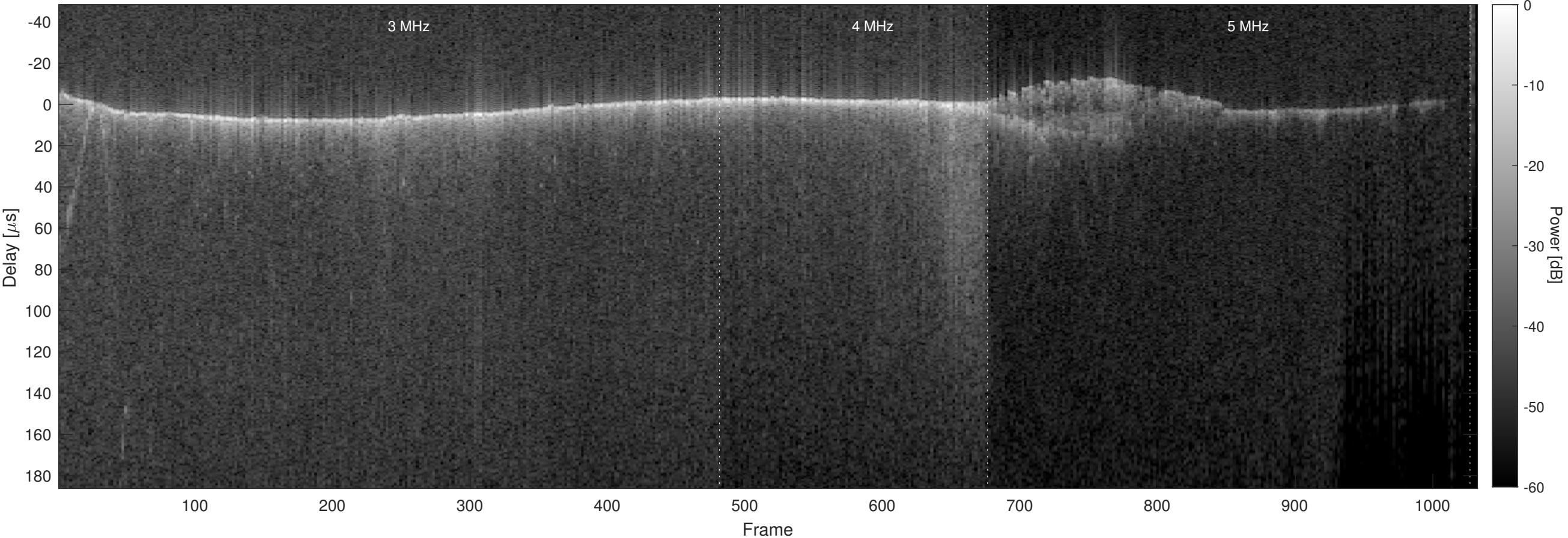
Orbit 9932, Optimized, No Window, Channel 2
