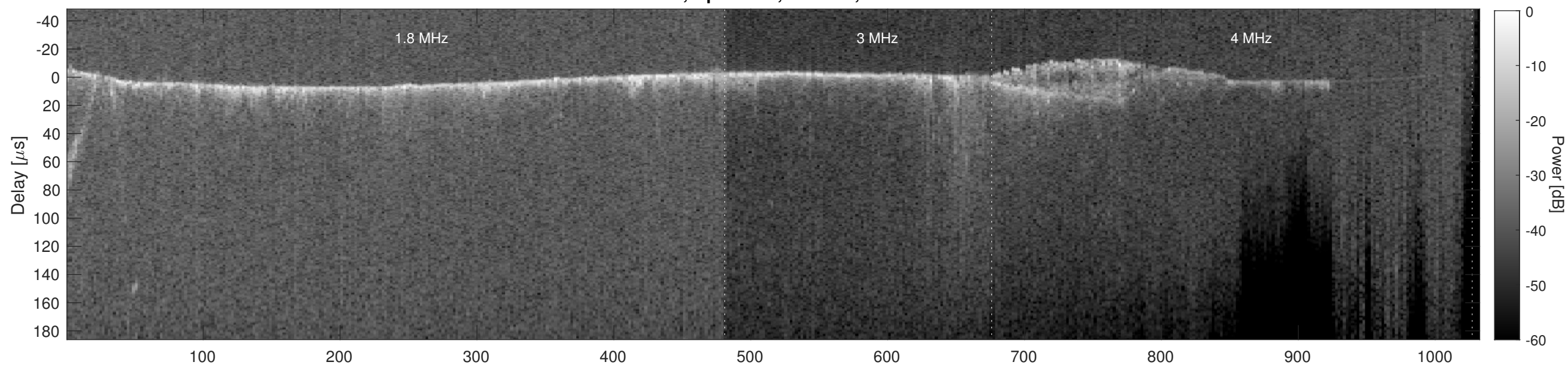
Orbit 9932, Cluttergram
