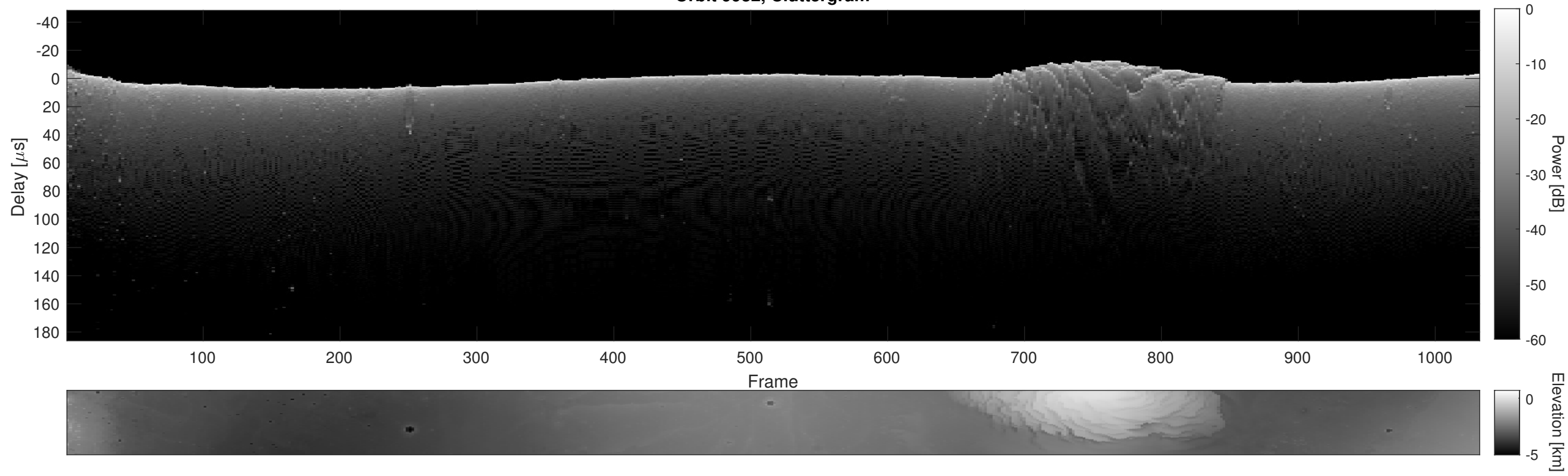
Orbit 9932, Cluttergram
