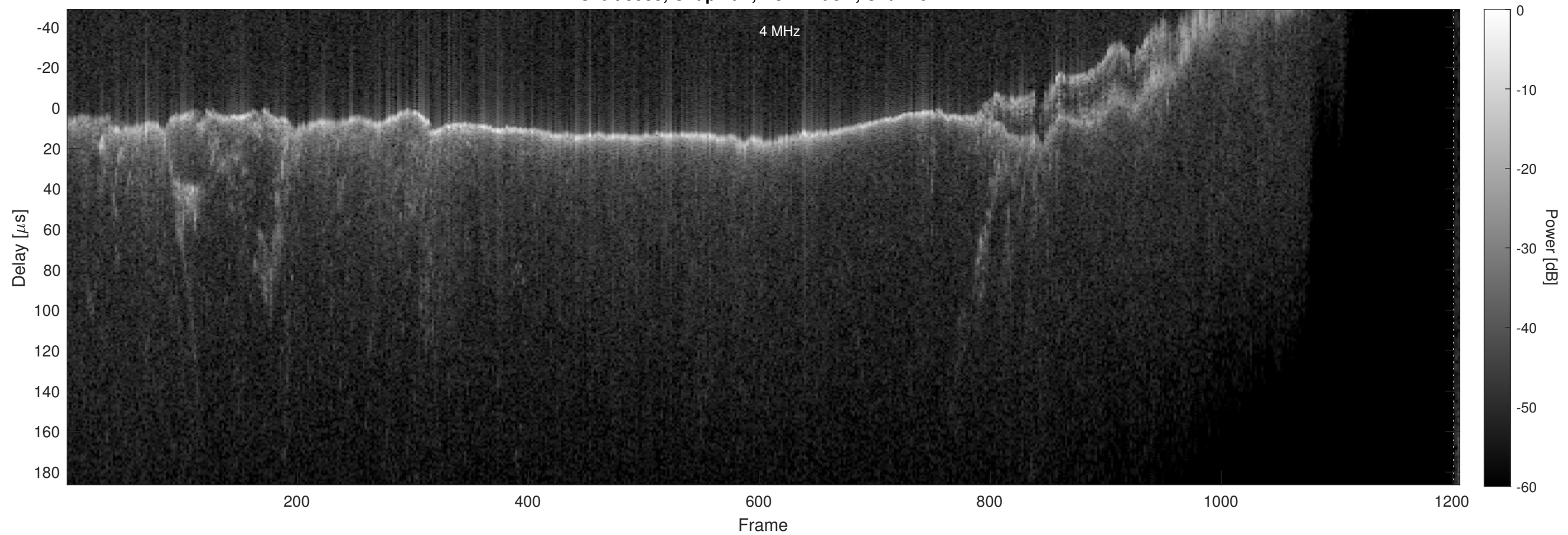
Orbit 9933, Chapman, No Window, Channel 2
