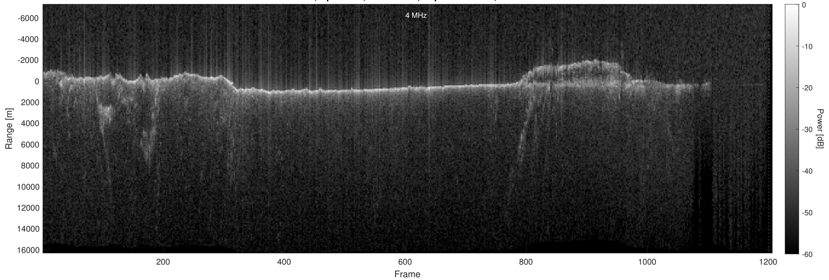
Orbit 9933, Optimized, No Window, Depth-Corrected, Channel 2
