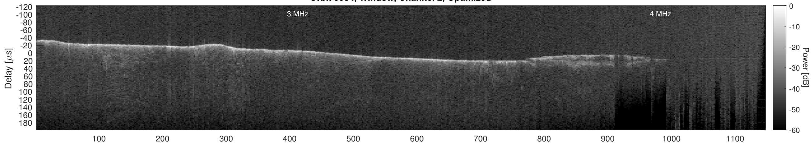
Orbit 9934, Cluttergram
