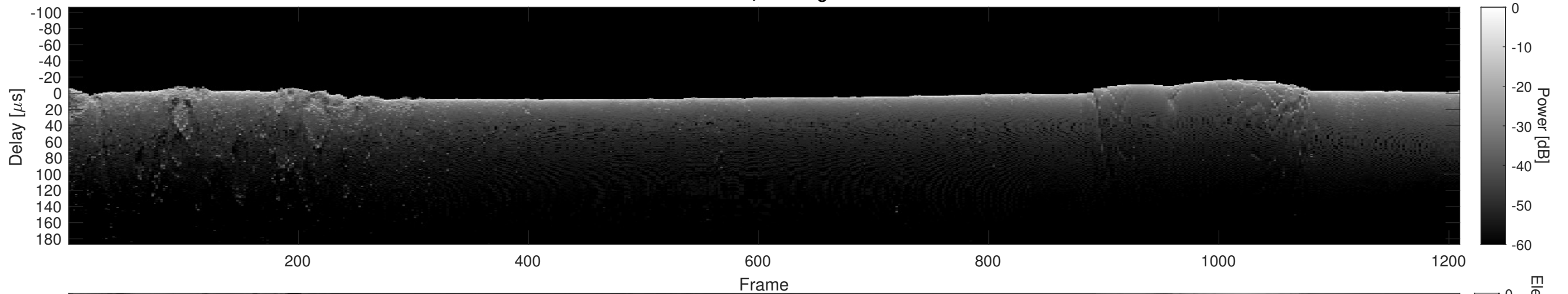
Orbit 9986, Cluttergram
