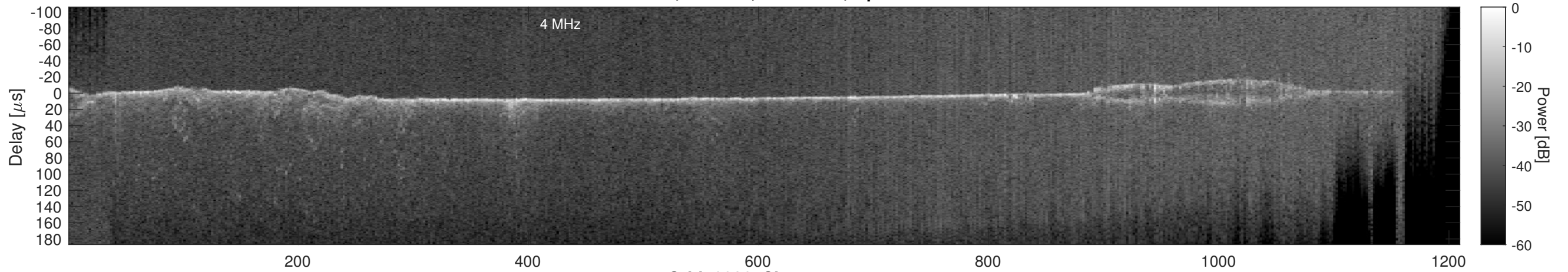
Orbit 9986, Cluttergram
