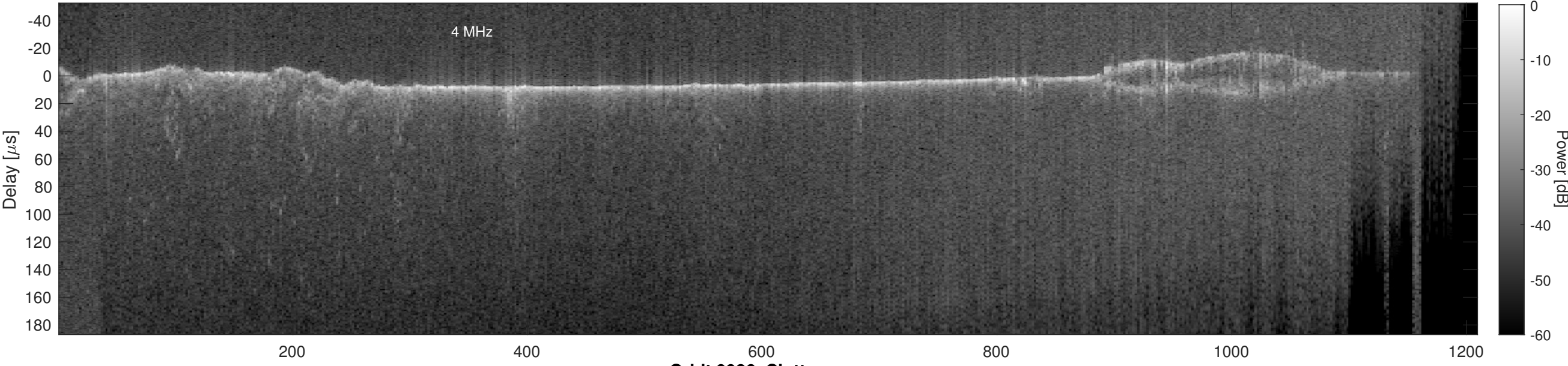
Orbit 9986, Cluttergram
