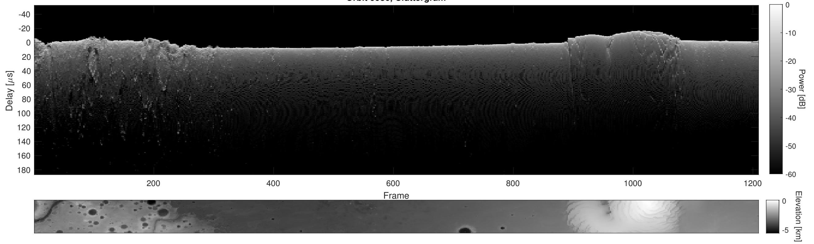
Orbit 9986, Cluttergram
