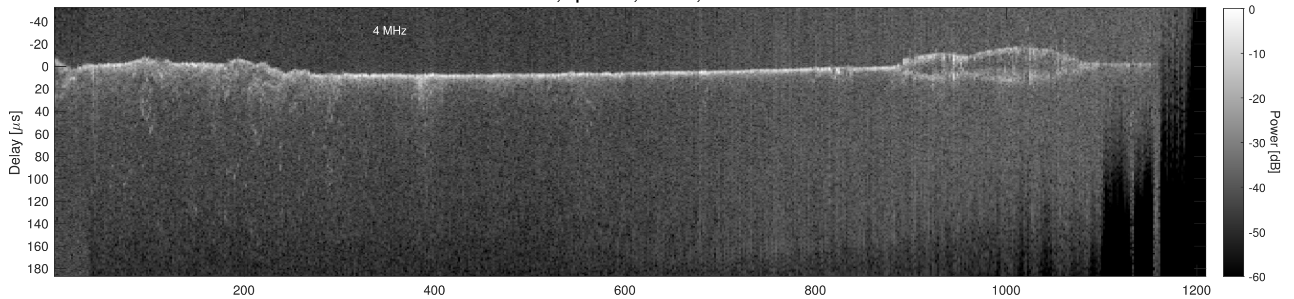
Orbit 9986, Cluttergram
