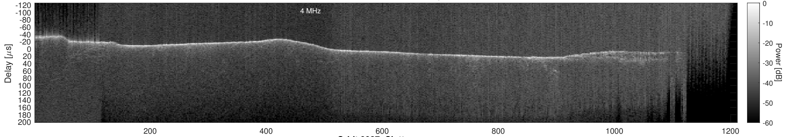
Orbit 9987, Cluttergram
