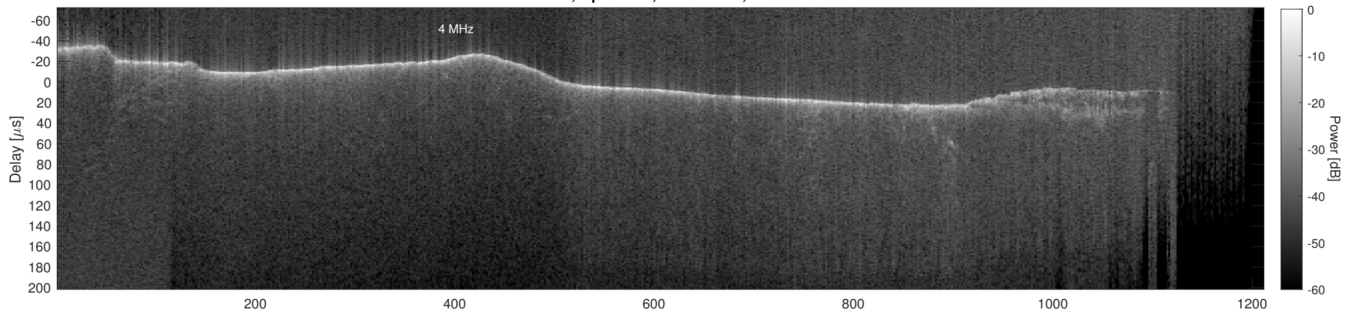
Orbit 9987, Cluttergram
