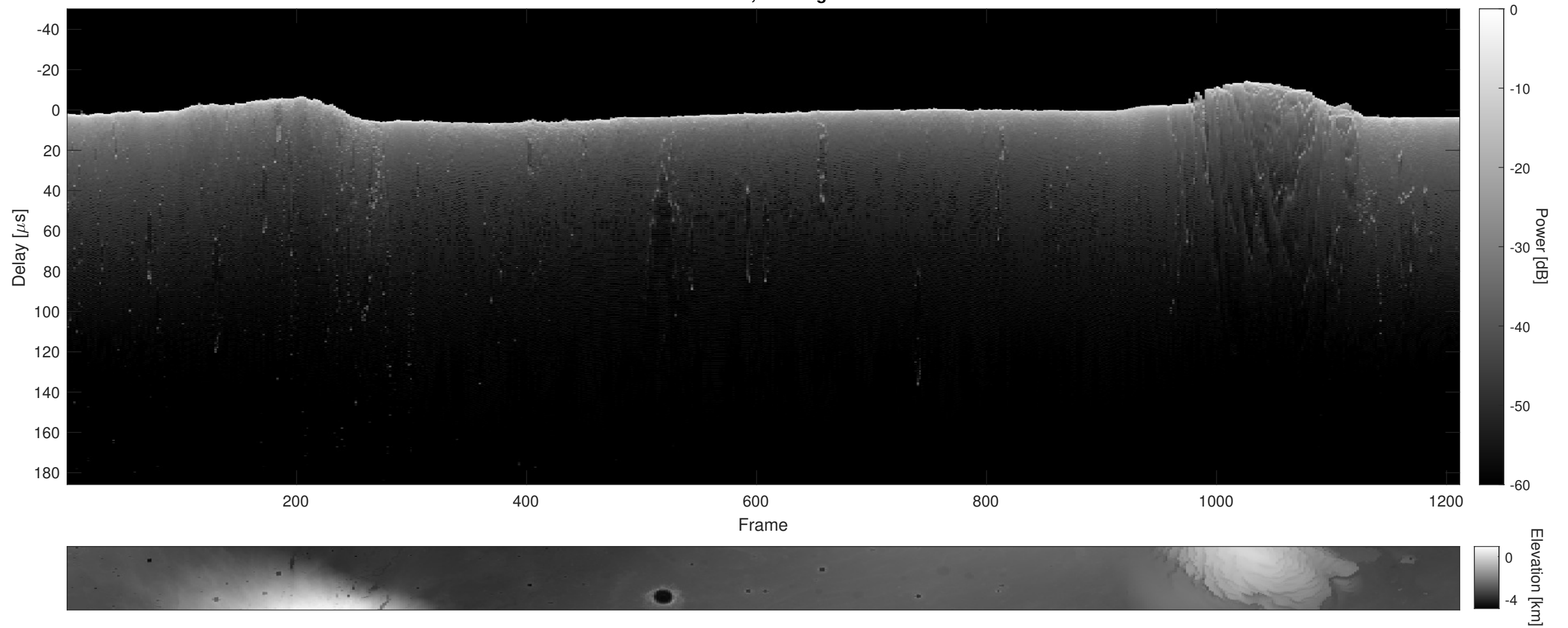
Orbit 9988, Cluttergram
