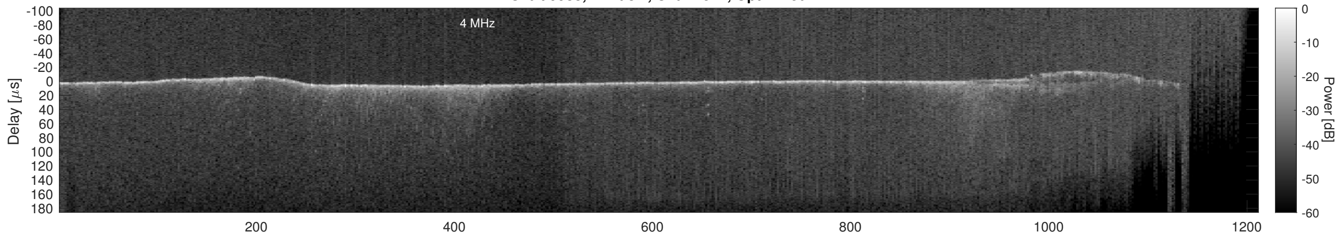
Orbit 9988, Cluttergram
