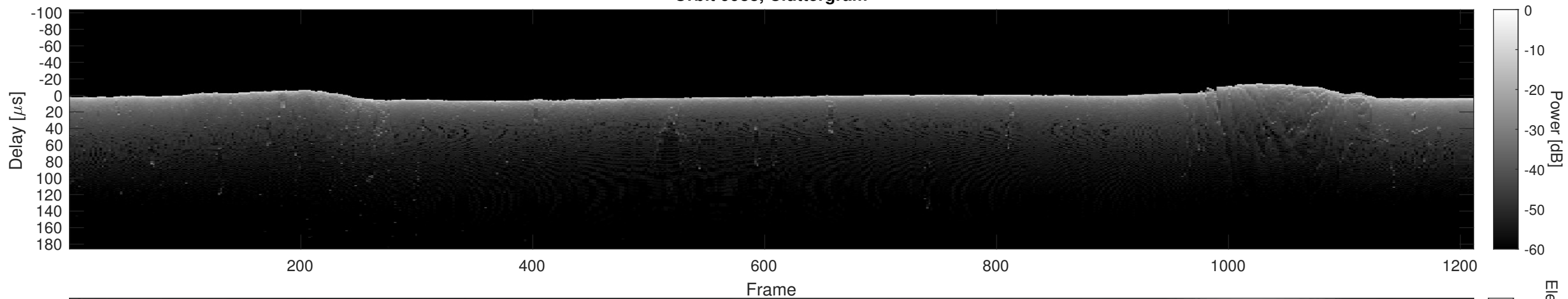
Orbit 9988, Cluttergram
