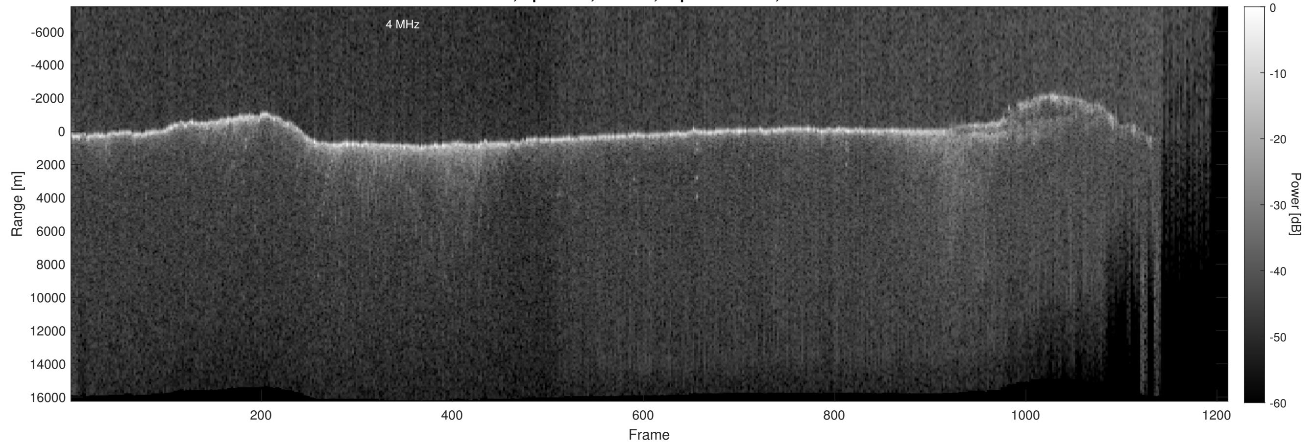
Orbit 9988, Optimized, Window, Depth-Corrected, Channel 2
