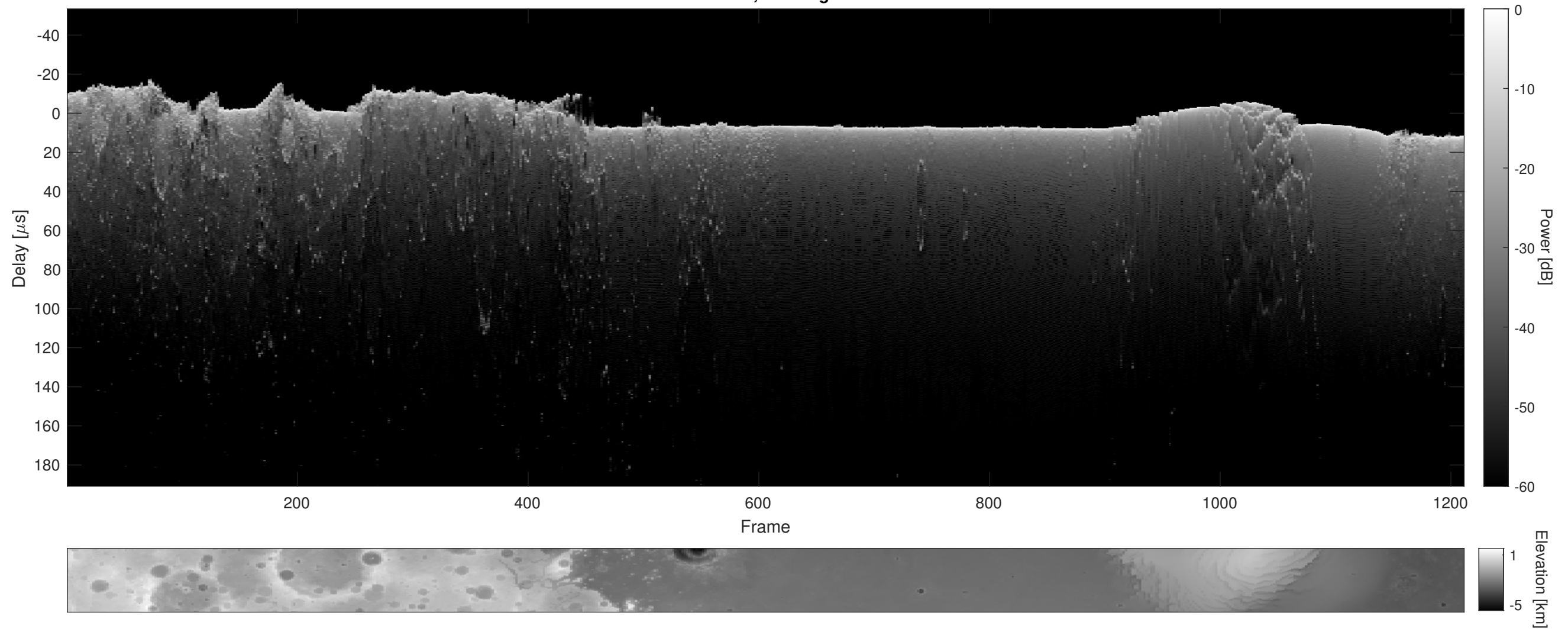
Orbit 9989, Cluttergram
