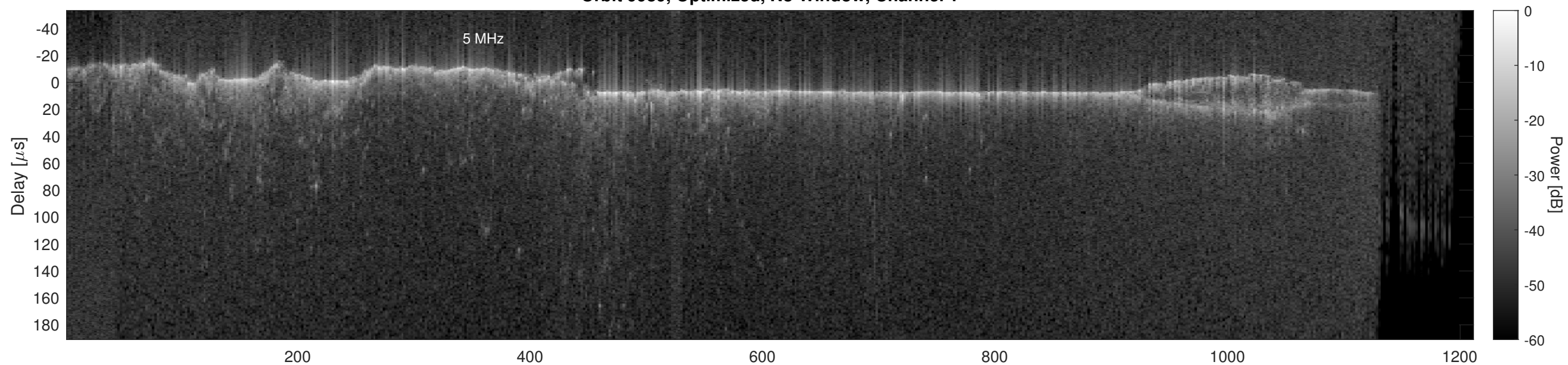
Orbit 9989, Optimized, No Window, Channel 2
