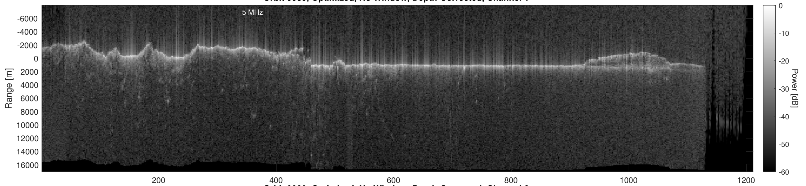
Orbit 9989, Optimized, No Window, Depth-Corrected, Channel 2
