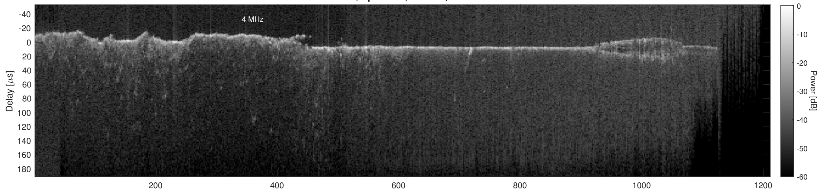
Orbit 9989, Cluttergram
