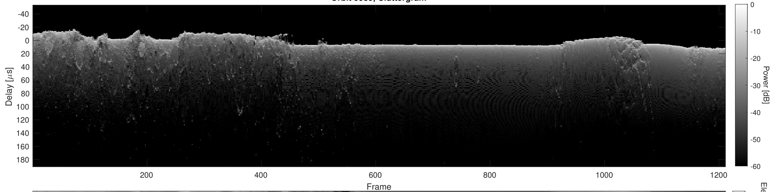
Orbit 9989, Cluttergram
