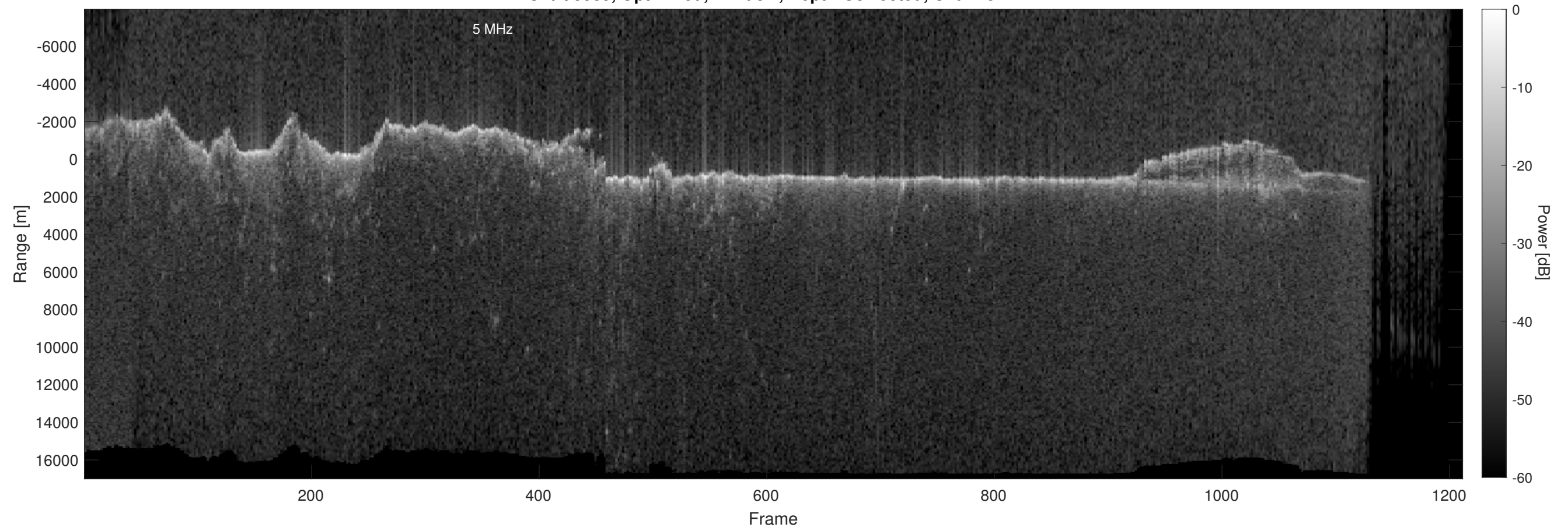
Orbit 9989, Optimized, Window, Depth-Corrected, Channel 2
