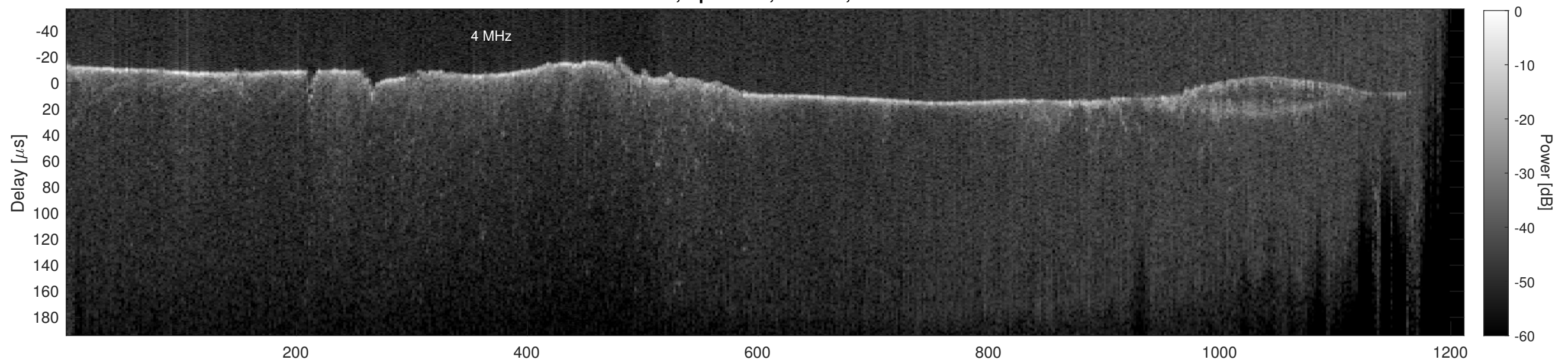
Orbit 9990, Cluttergram
