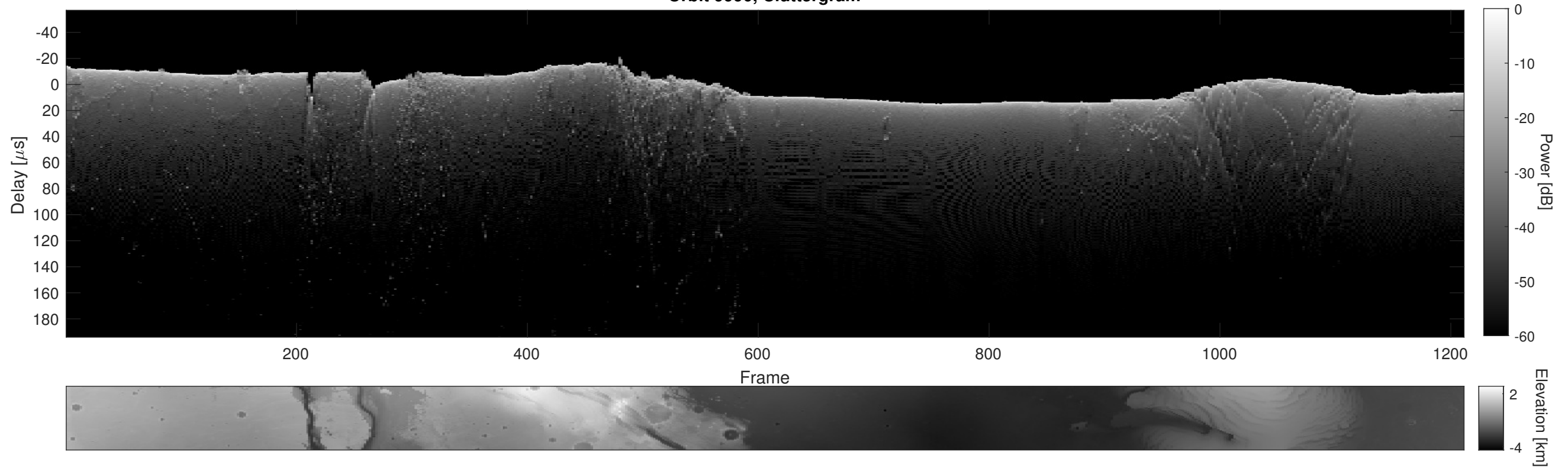
Orbit 9990, Cluttergram
