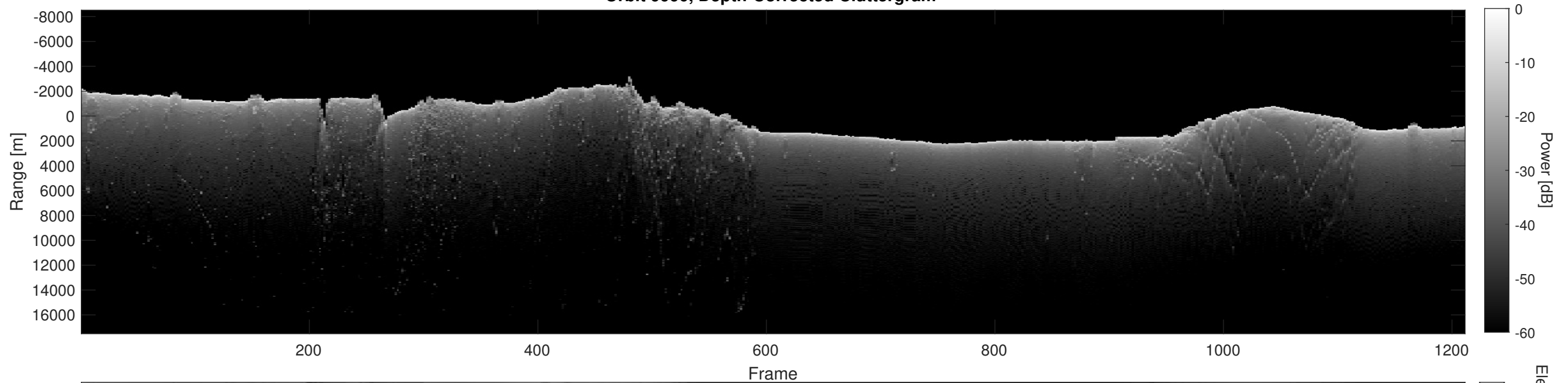
Orbit 9990, Depth-Corrected Cluttergram
