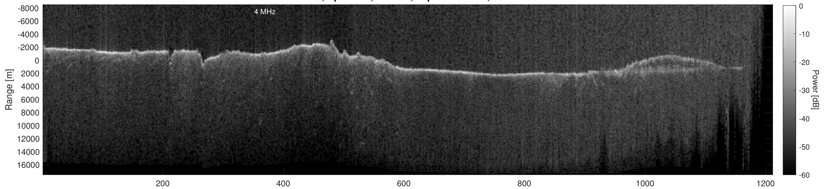
Orbit 9990, Depth-Corrected Cluttergram
