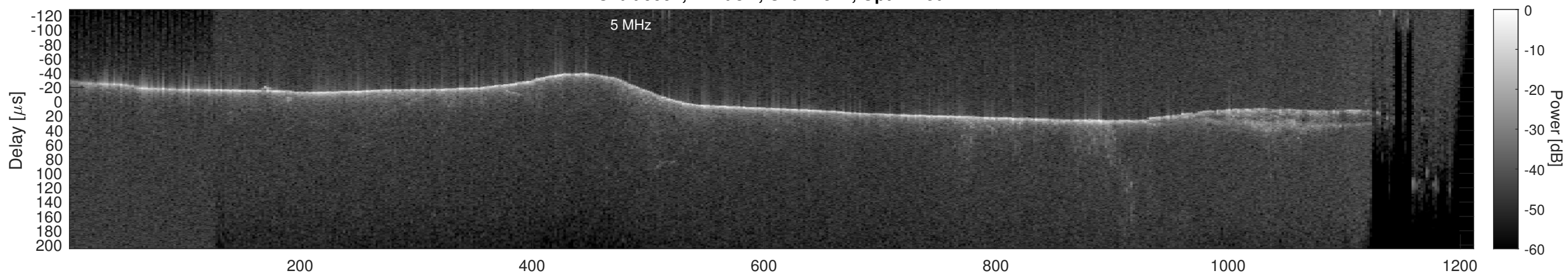
Orbit 9994, Cluttergram
