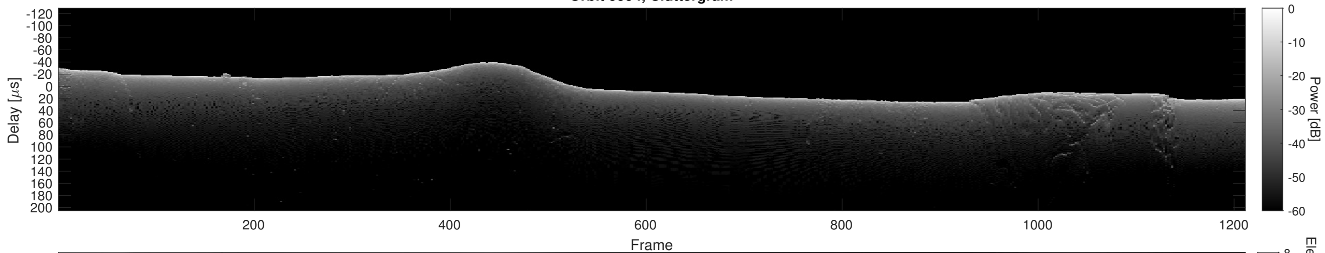
Orbit 9994, Cluttergram
