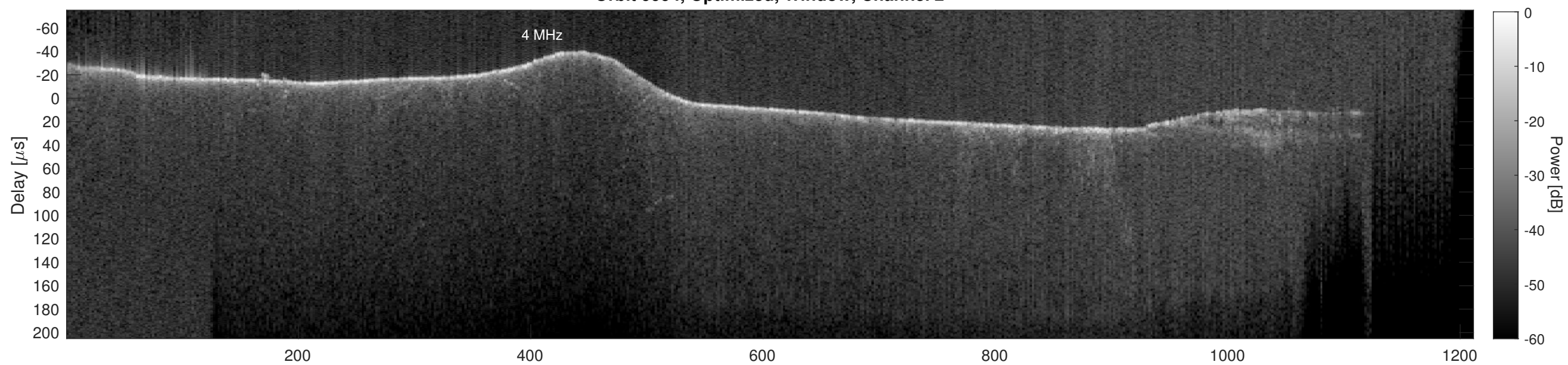
Orbit 9994, Cluttergram
