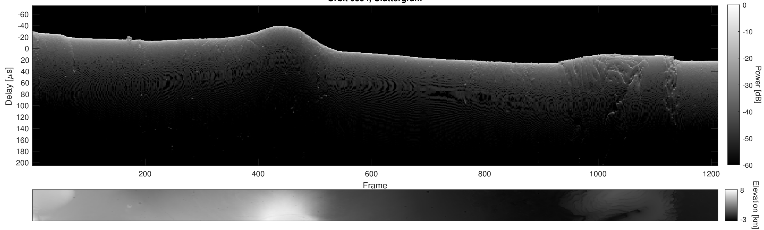
Orbit 9994, Cluttergram
