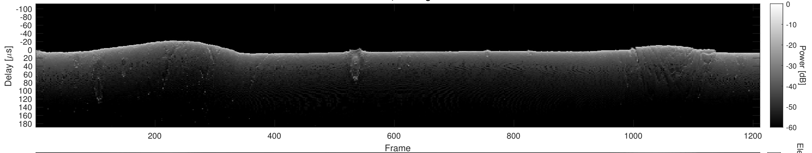
Orbit 9995, Cluttergram
