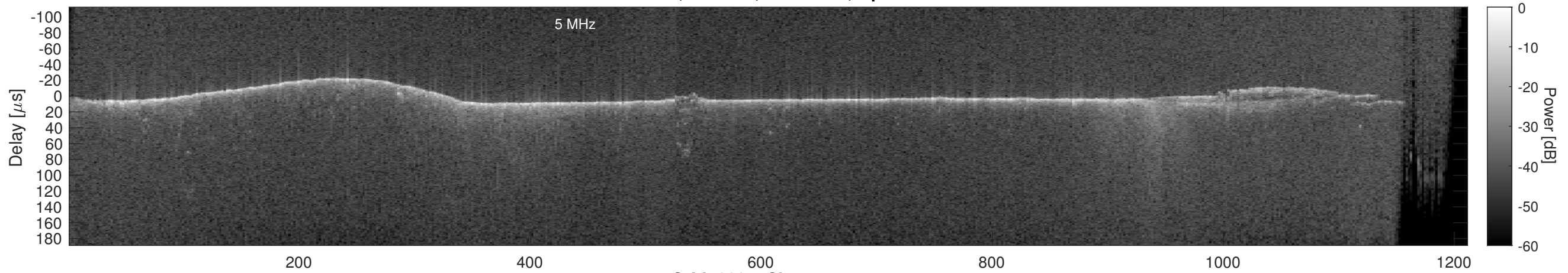
Orbit 9995, Cluttergram
