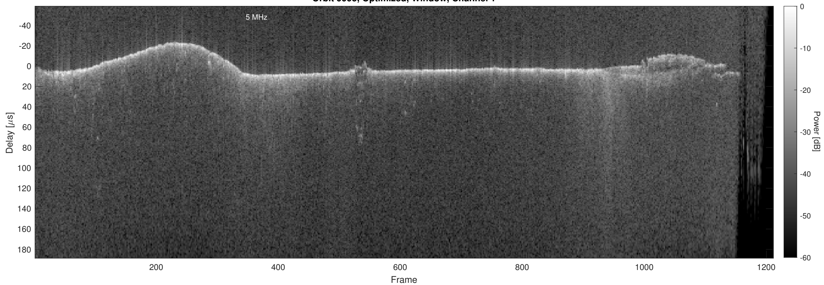
Orbit 9995, Optimized, Window, Channel 2
