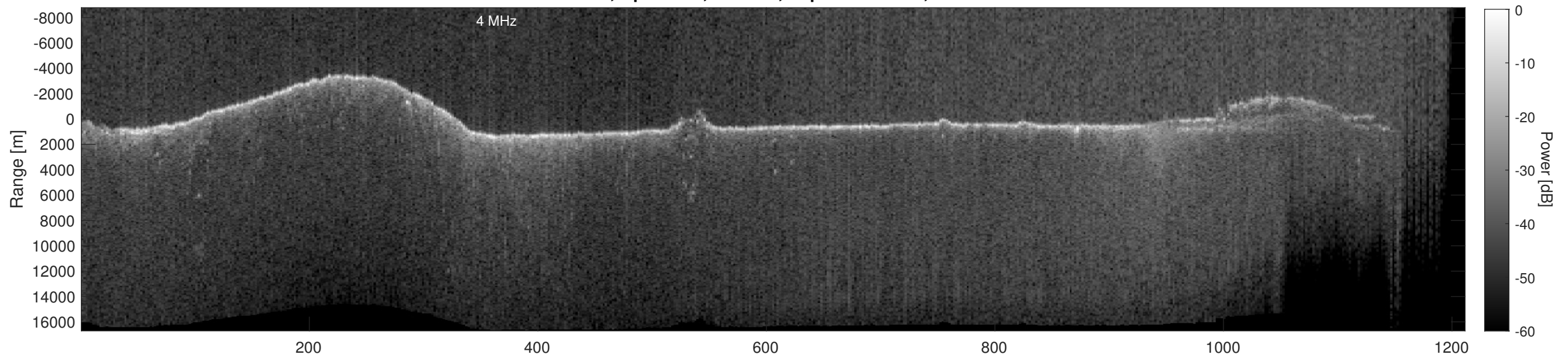
Orbit 9995, Depth-Corrected Cluttergram
