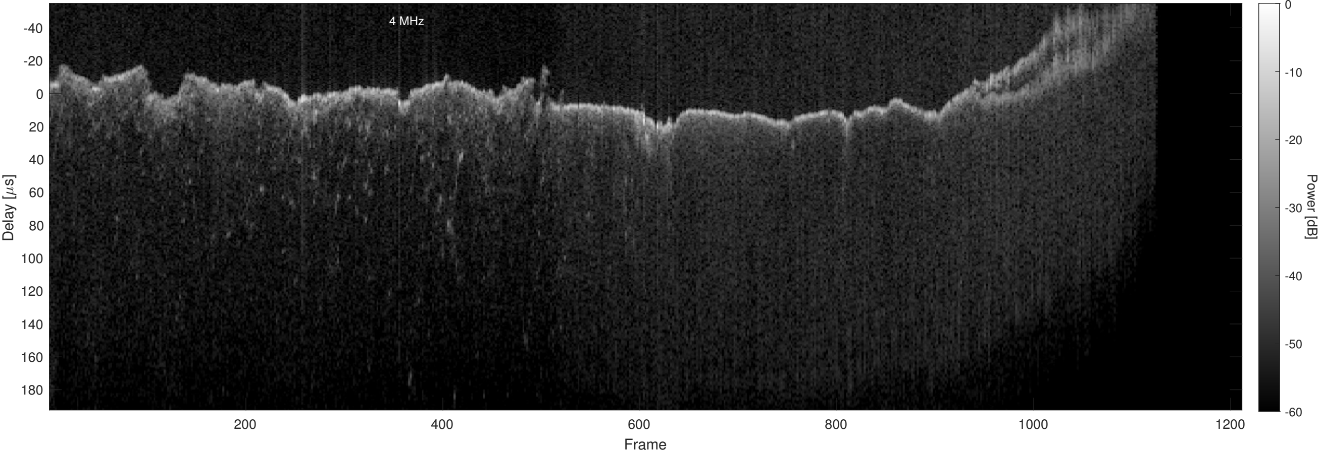
Orbit 9996, Chapman, Window, Channel 2
