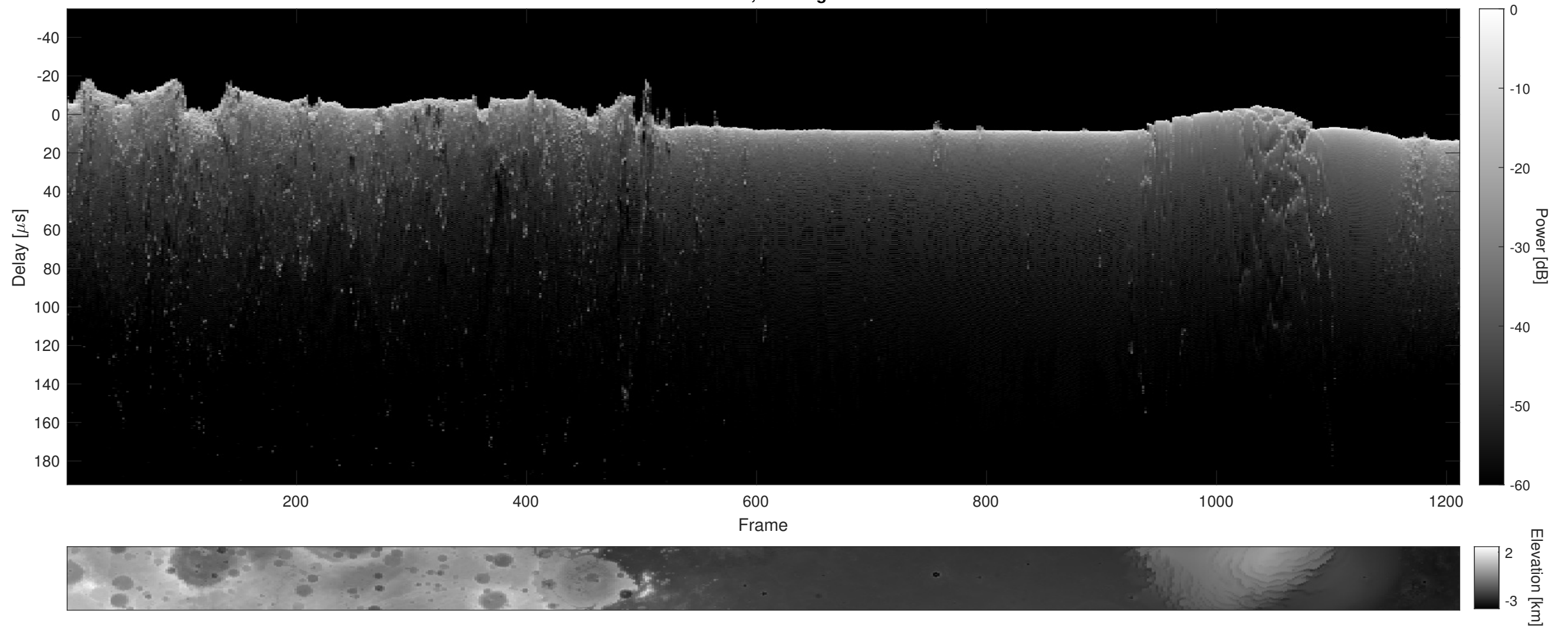
Orbit 9996, Cluttergram
