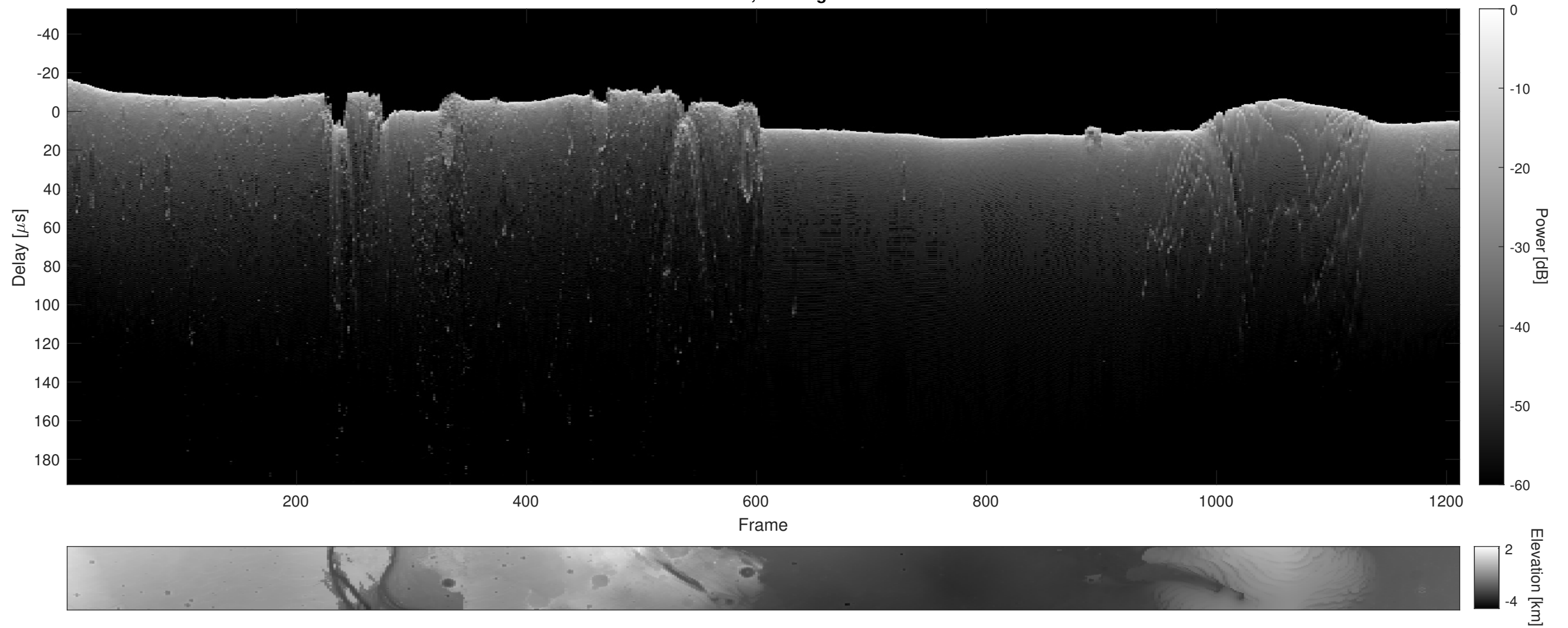
Orbit 9997, Cluttergram
