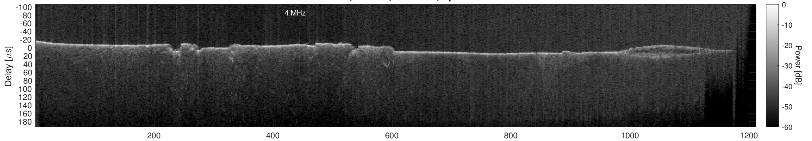
Orbit 9997, Cluttergram
