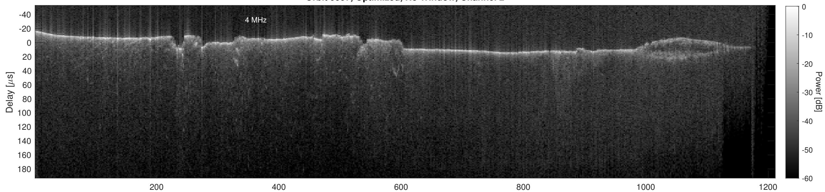
Orbit 9997, Cluttergram
