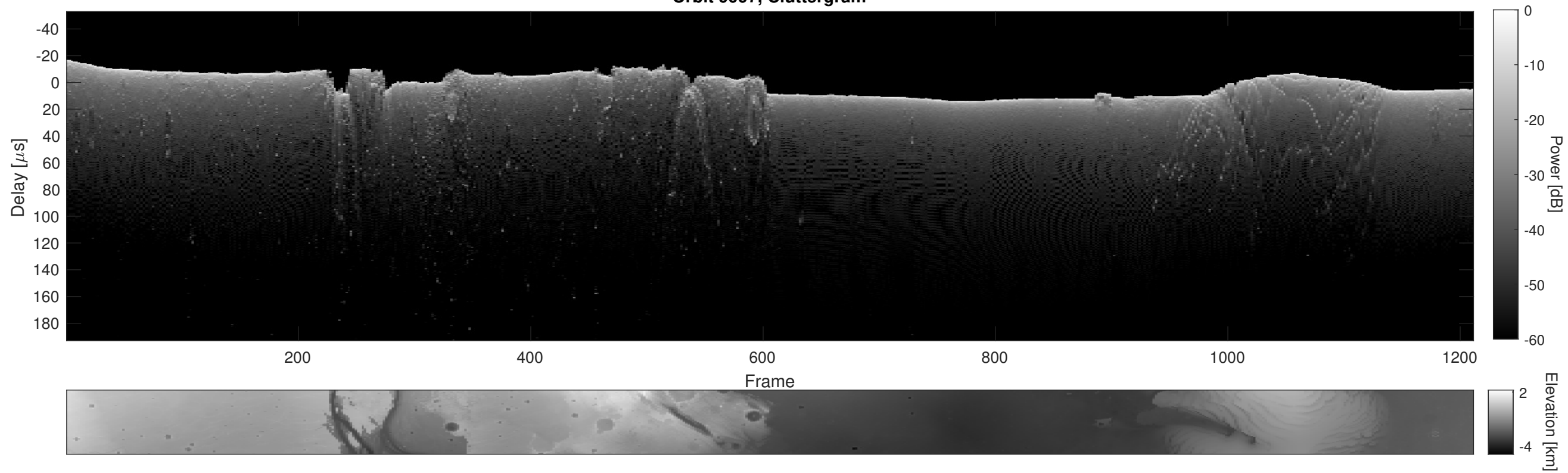
Orbit 9997, Cluttergram
