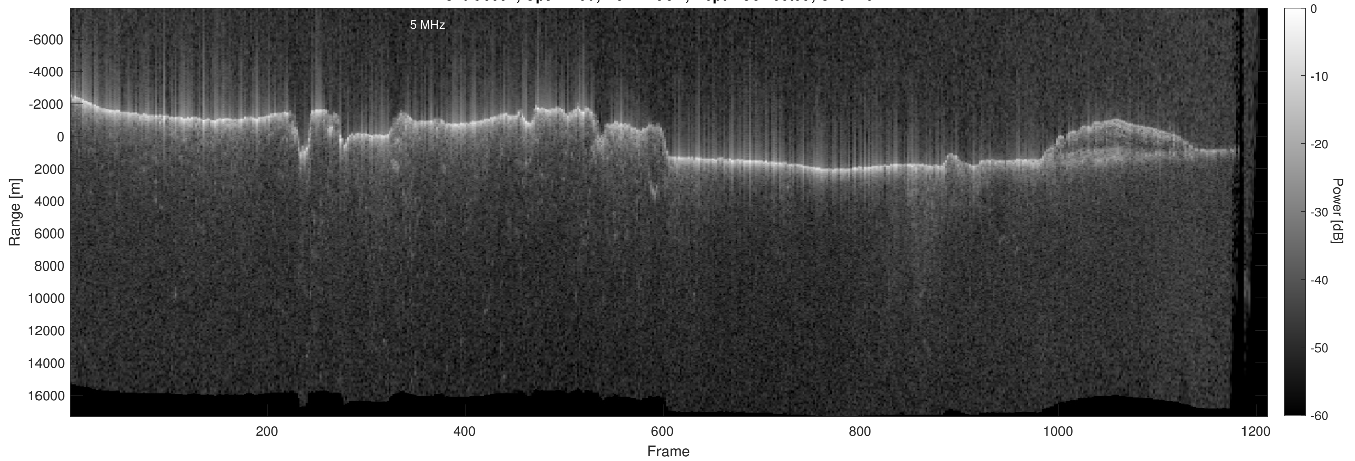
Orbit 9997, Optimized, No Window, Depth-Corrected, Channel 2
