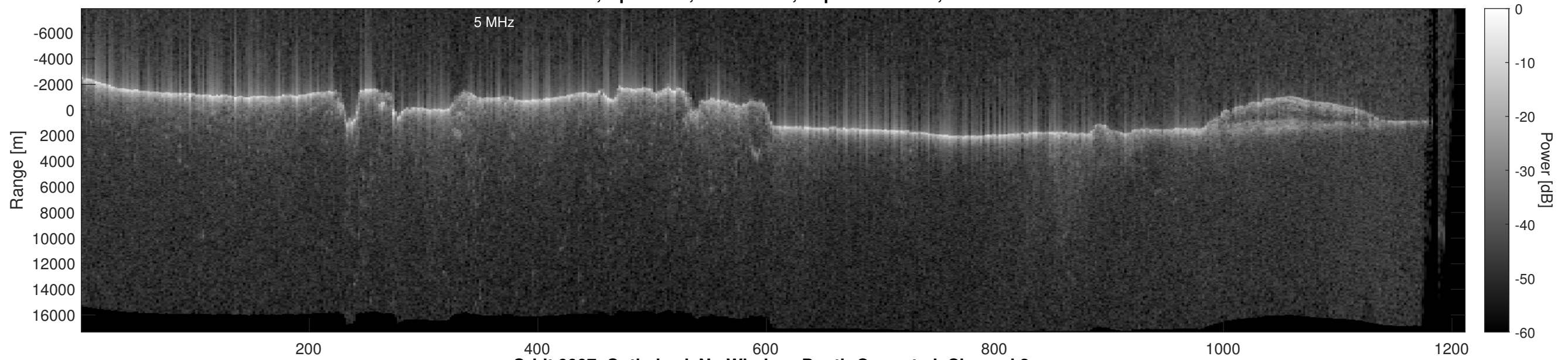
Orbit 9997, Optimized, No Window, Depth-Corrected, Channel 2
