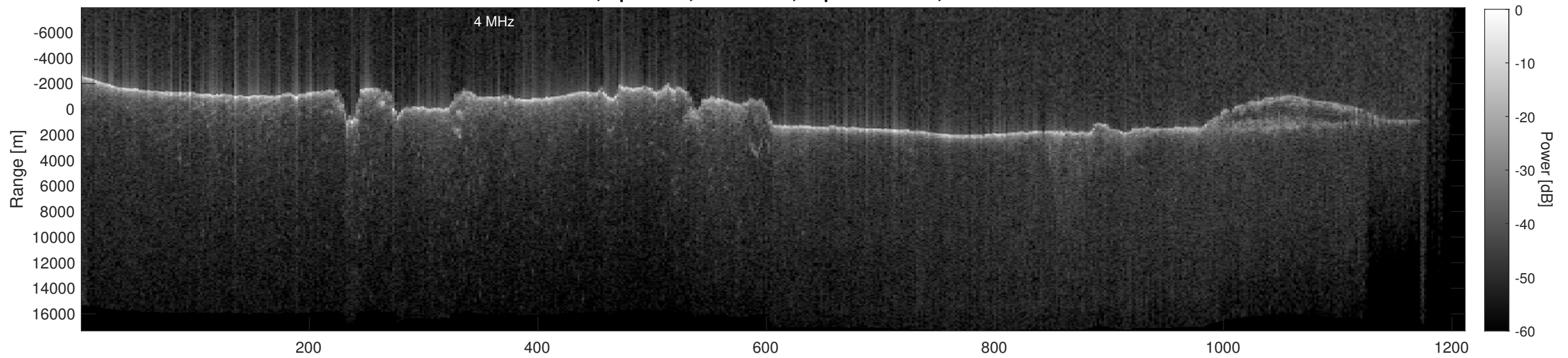
Orbit 9997, Depth-Corrected Cluttergram
