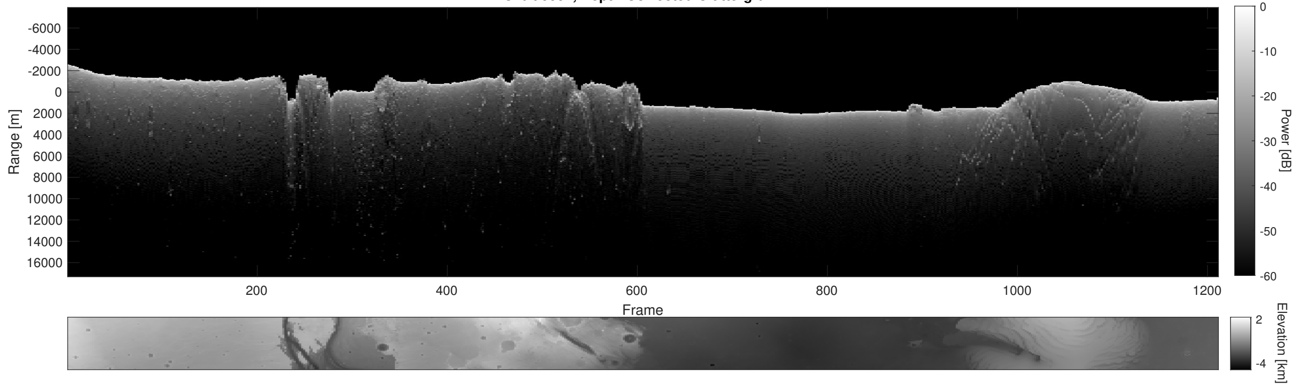
Orbit 9997, Depth-Corrected Cluttergram
