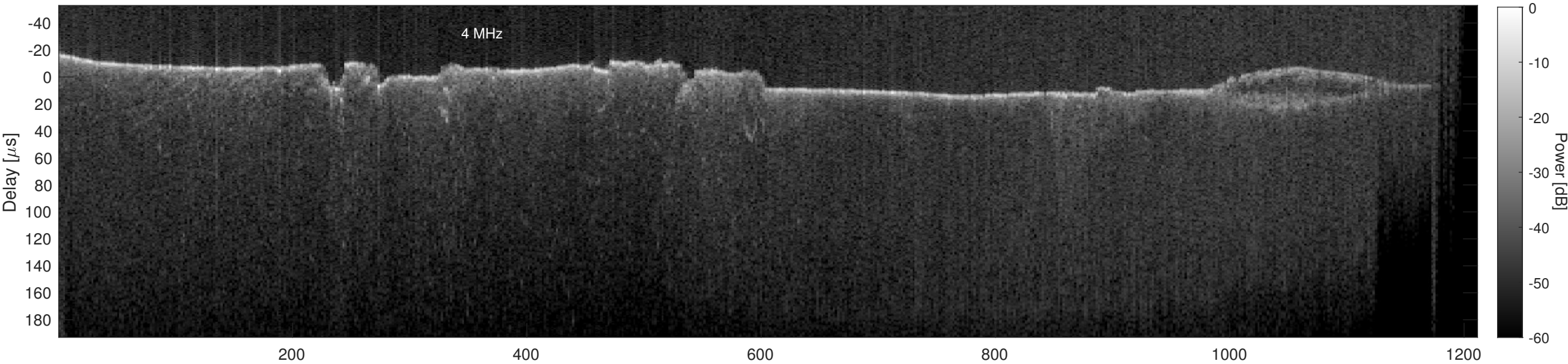
Orbit 9997, Cluttergram
