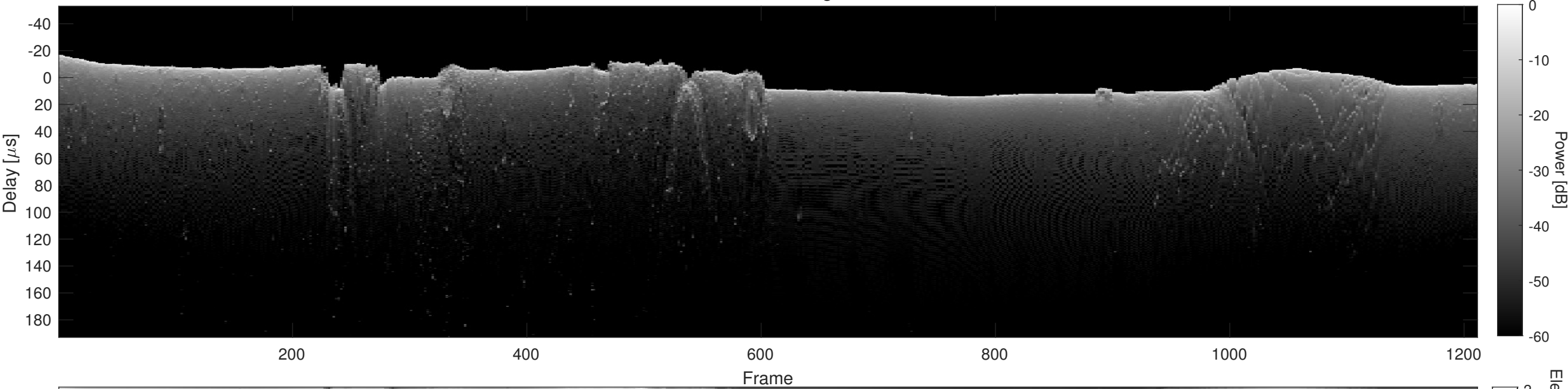
Orbit 9997, Cluttergram
