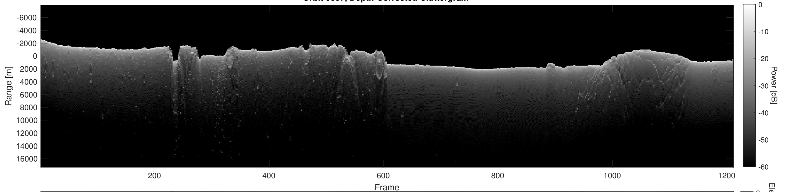
Orbit 9997, Depth-Corrected Cluttergram
