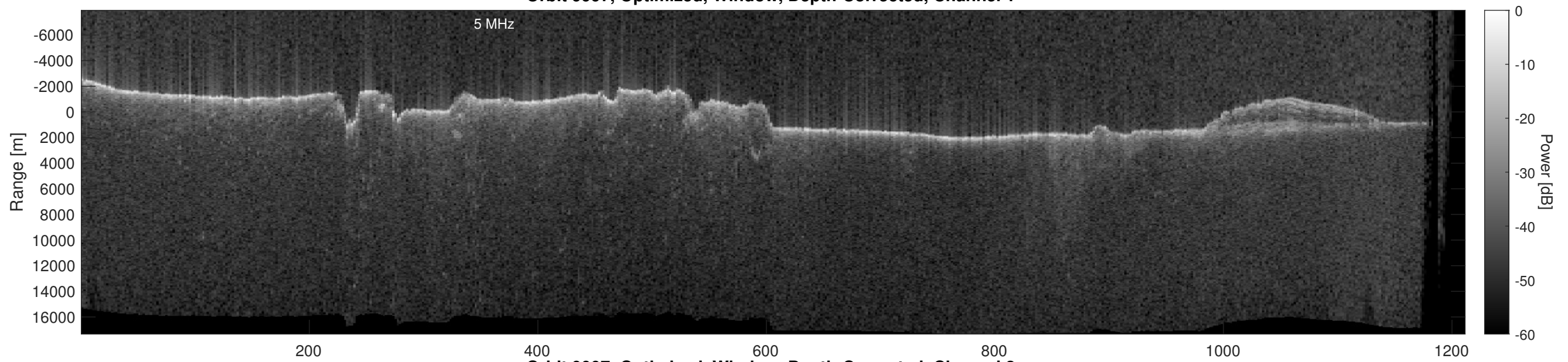
Orbit 9997, Optimized, Window, Depth-Corrected, Channel 2
