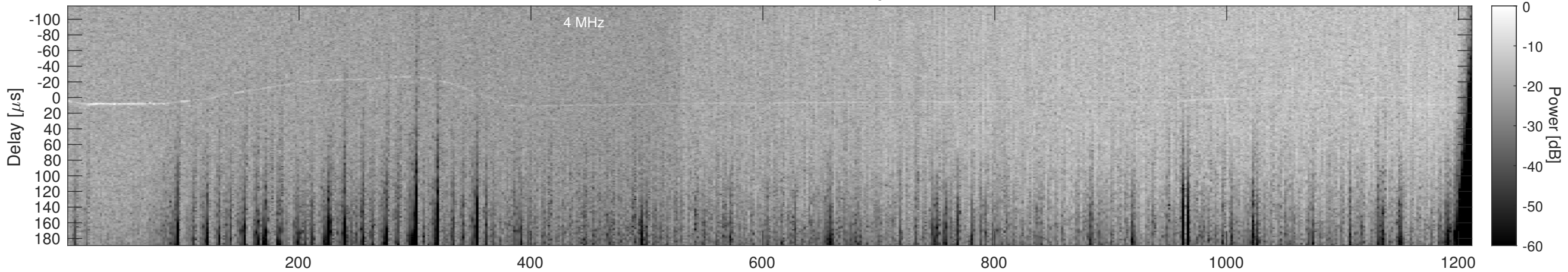
Orbit 10002, Cluttergram
