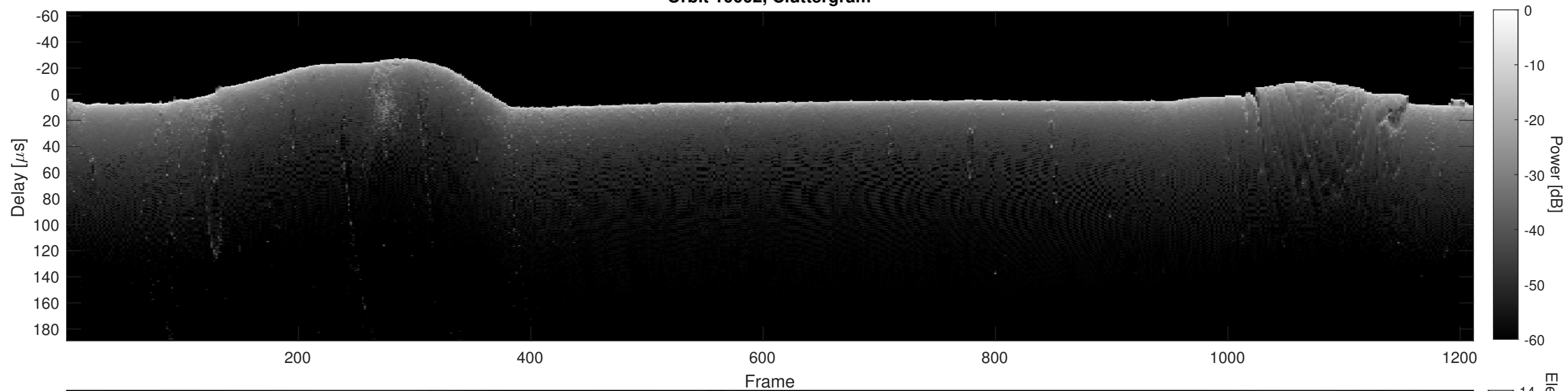
Orbit 10002, Cluttergram
