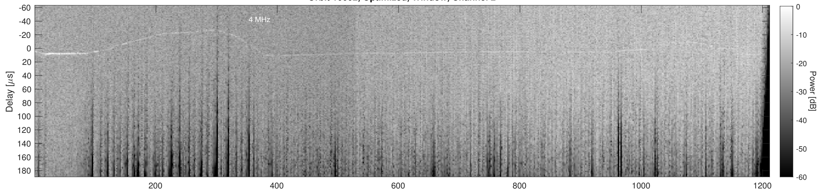
Orbit 10002, Cluttergram
