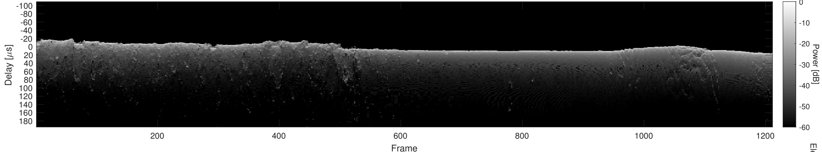
Orbit 10003, Cluttergram
