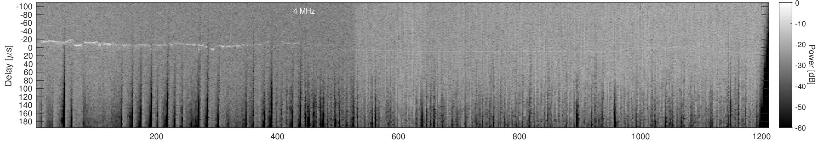
Orbit 10003, Cluttergram
