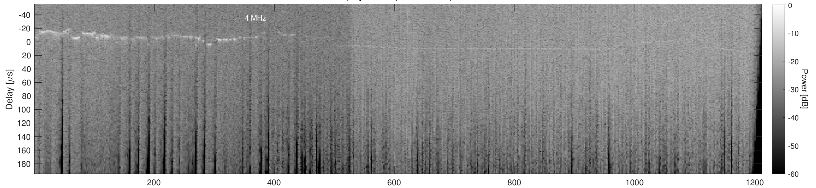
Orbit 10003, Cluttergram
