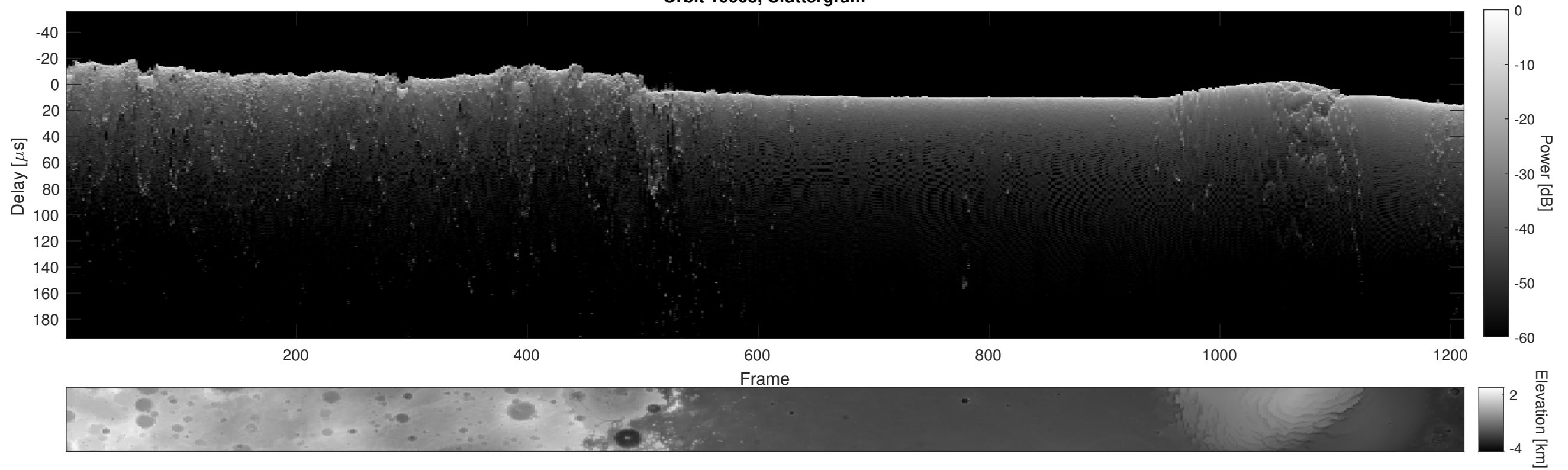
Orbit 10003, Cluttergram
