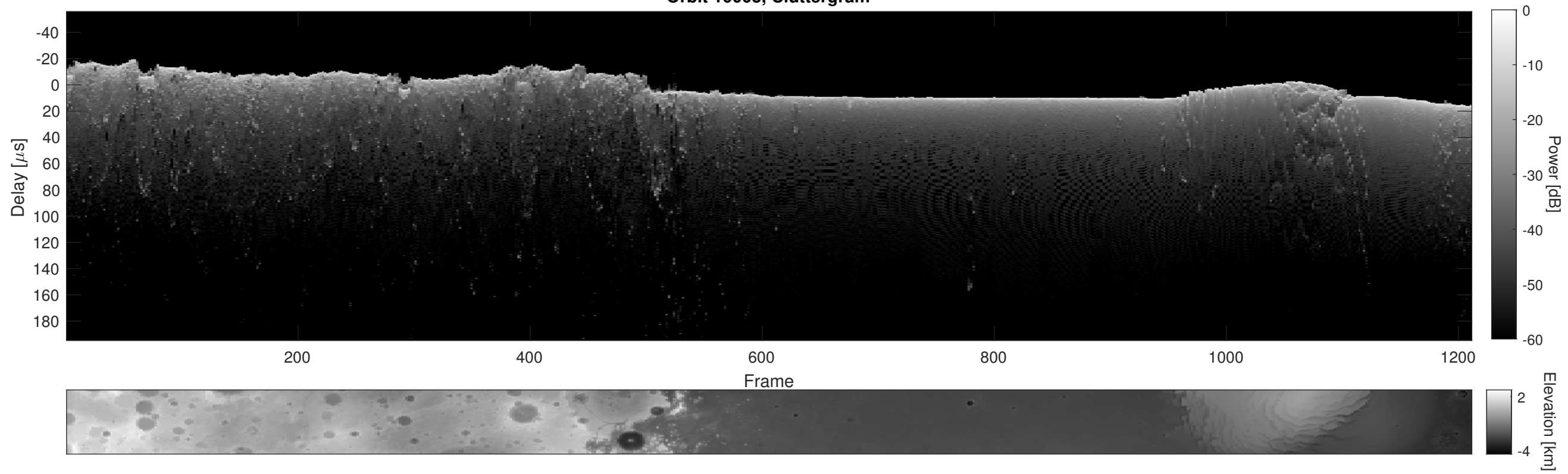
Orbit 10003, Cluttergram
