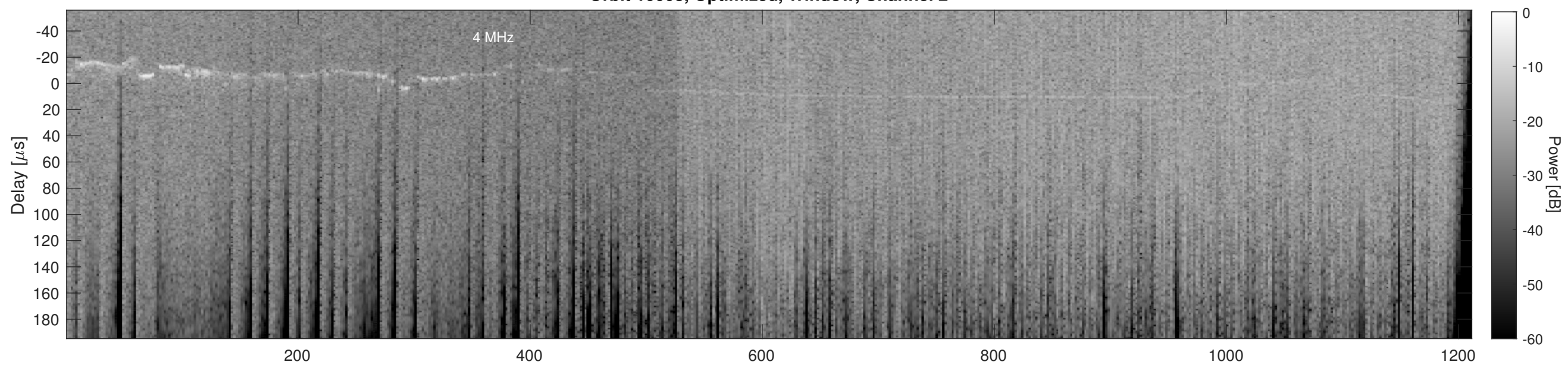
Orbit 10003, Cluttergram
