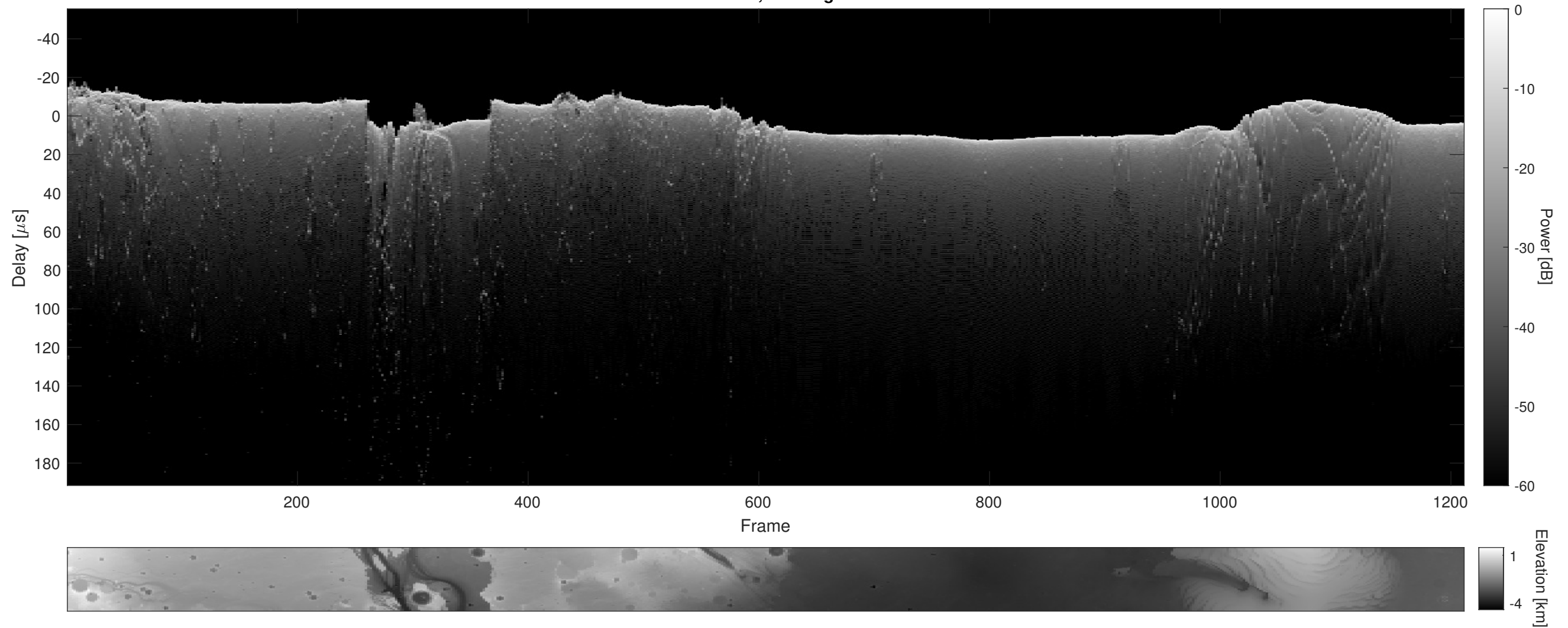
Orbit 10004, Cluttergram
