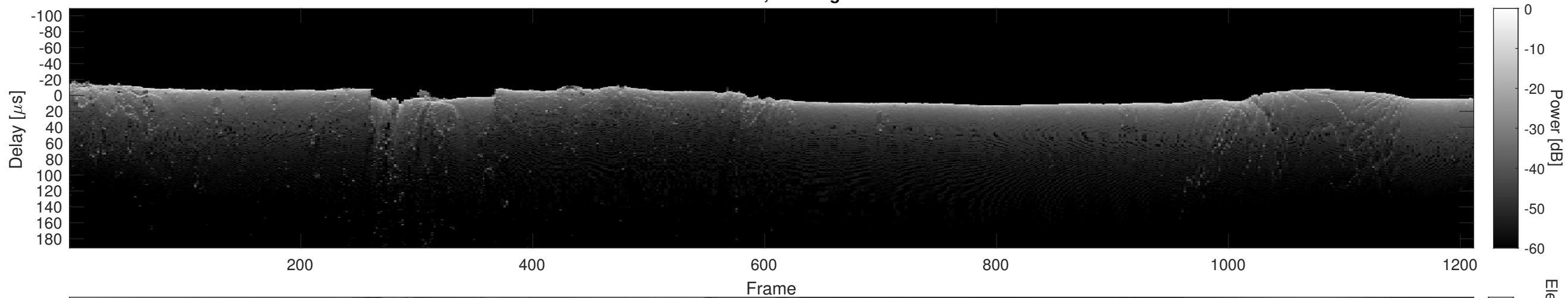
Orbit 10004, Cluttergram
