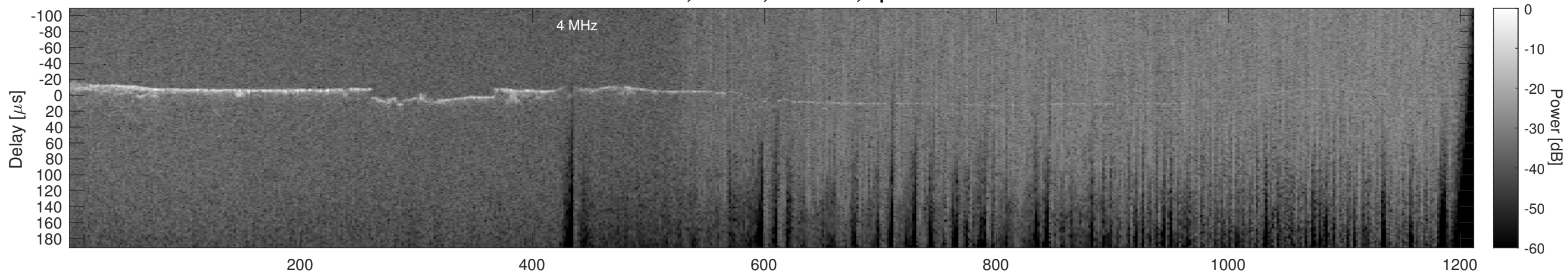
Orbit 10004, Cluttergram
