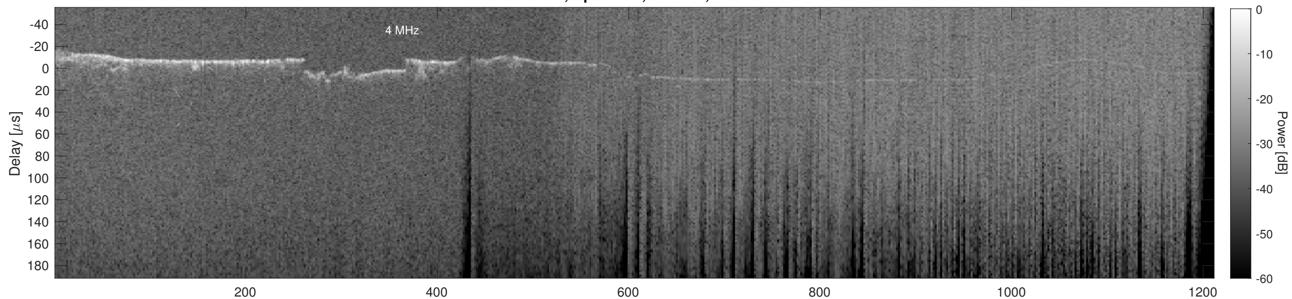
Orbit 10004, Cluttergram
